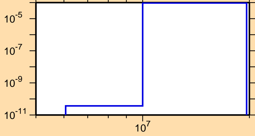
\sigma vs. E for ^{210}\text{Po}(n,t)
