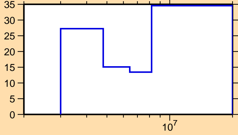
\Delta\sigma/\sigma vs. E for ^{210}\text{Po}(n,n\text{cont.})
