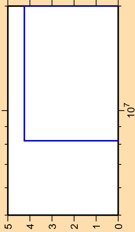
\Delta\sigma/\sigma vs. E for ^{210}\text{Po}(n,\text{pd})
