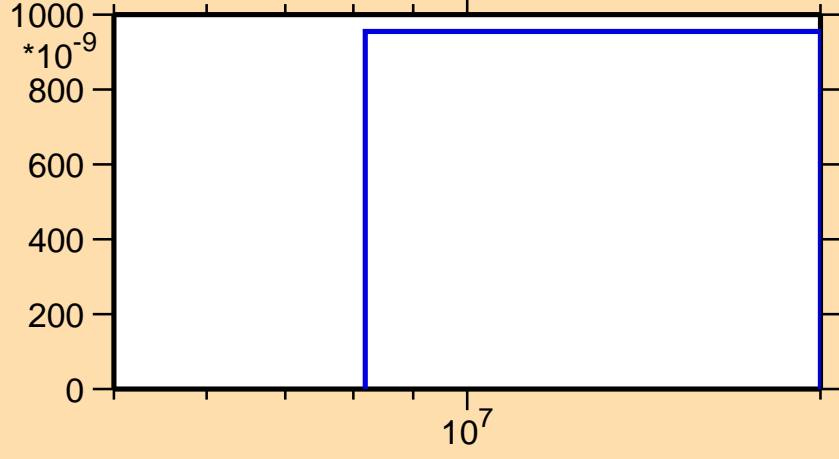
\sigma vs. E for ^{210}\text{Po}(n,2n\alpha)
