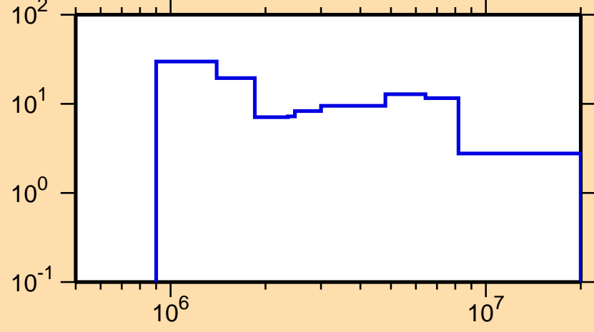
\Delta\sigma/\sigma vs. E for ^{210}\text{Po}(n,\text{tot.})
