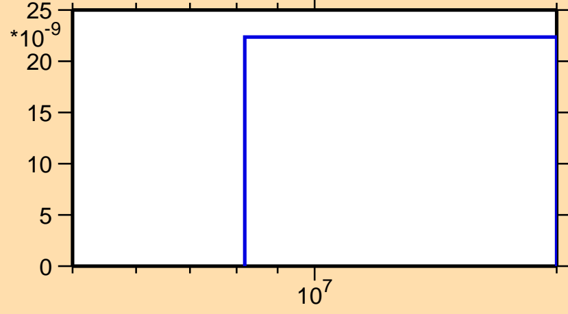
\sigma vs. E for ^{210}\text{Po}(n,2np)
