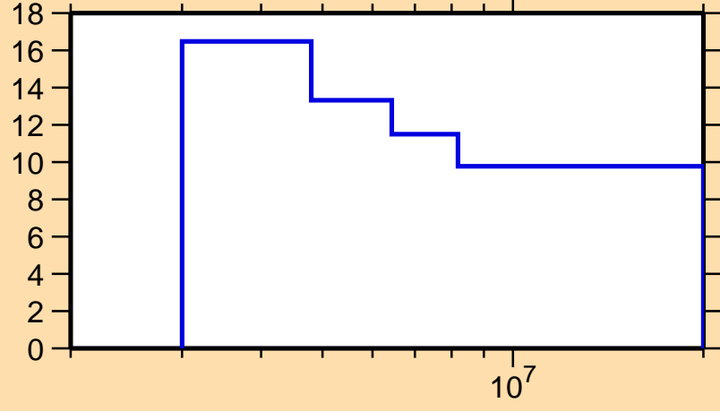
\Delta\sigma/\sigma vs. E for ^{210}\text{Po}(n,n\text{nonel.})
