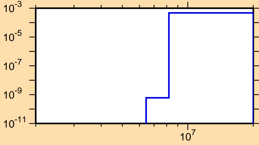
\sigma vs. E for ^{210}\text{Po}(n,d)
