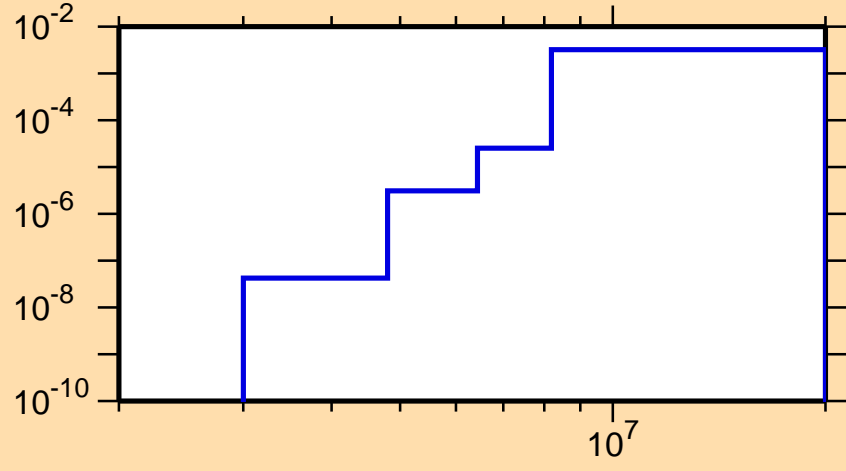
\sigma vs. E for ^{210}\text{Po}(n,p)
