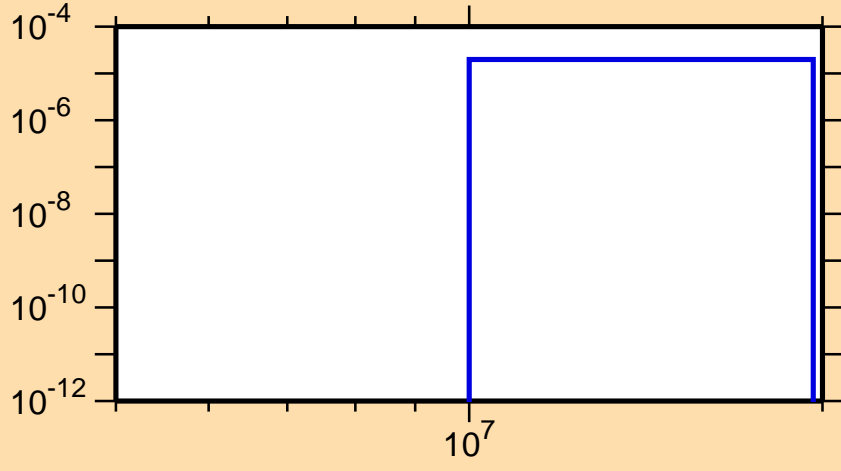
\sigma vs. E for ^{211}\text{Po}(n,\text{nd})
