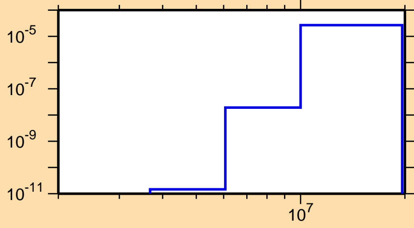
\sigma vs. E for ^{211}\text{Po}(n,2n\alpha)
