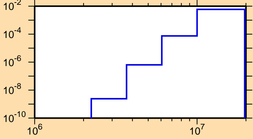
\sigma vs. E for ^{211}\text{Po}(n,p)
