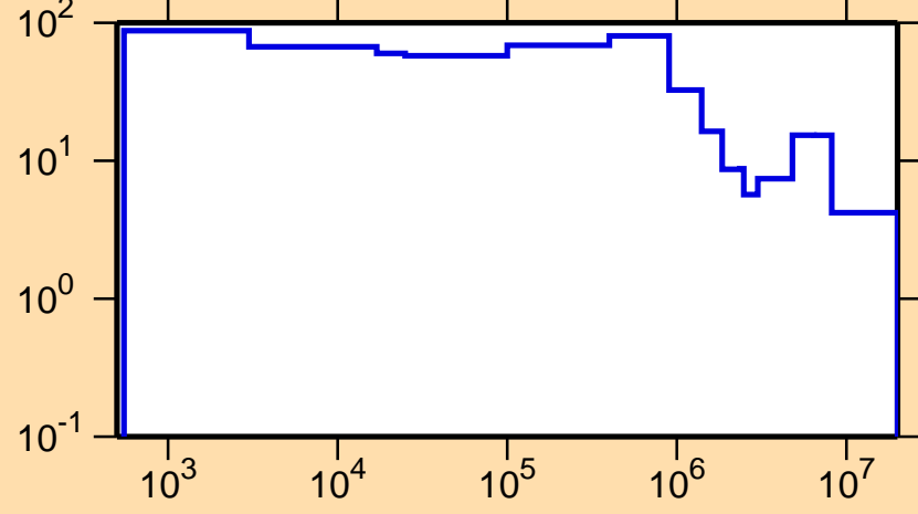
\Delta\sigma/\sigma vs. E for ^{211}\text{Po}(n,\text{tot.})
