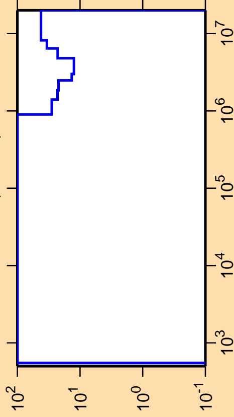
\Delta\sigma/\sigma vs. E for ^{211}\text{Po}(n,\text{inel.})
