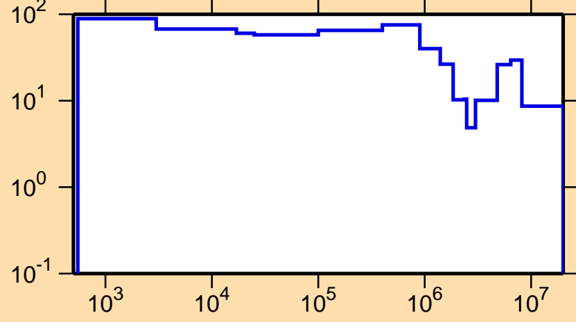
\Delta\sigma/\sigma vs. E for ^{211}\text{Po}(n,\text{el.})
