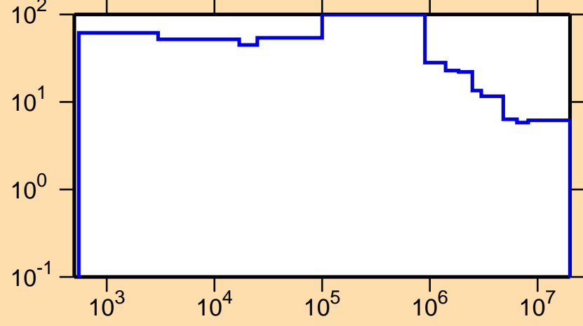
\Delta\sigma/\sigma vs. E for ^{211}\text{Po}(n,\text{nonel.})
