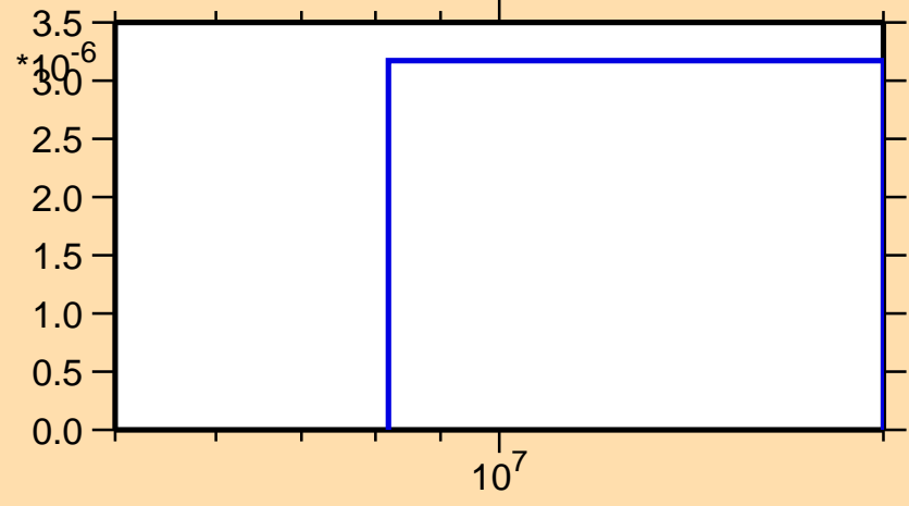
\sigma vs. E for ^{211}\text{Po}(n,\text{nt})
