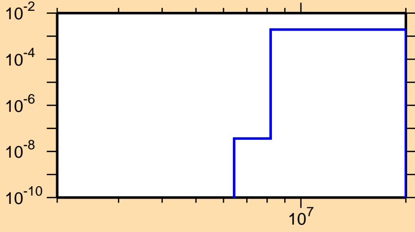
\sigma vs. E for ^{211}\text{Po}(n,d)
