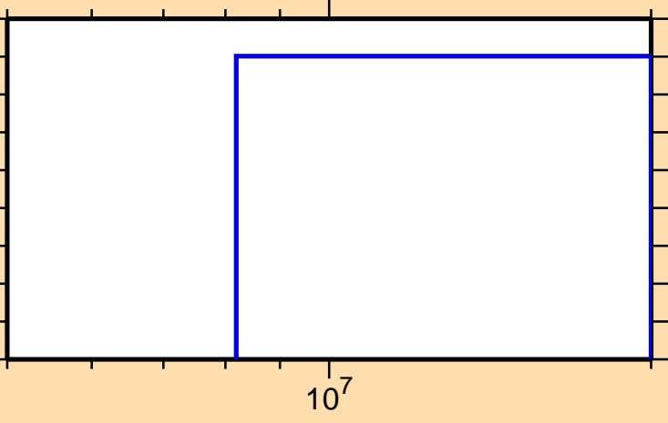
\sigma vs. E for ^{211}\text{Po}(n,\text{nd})
