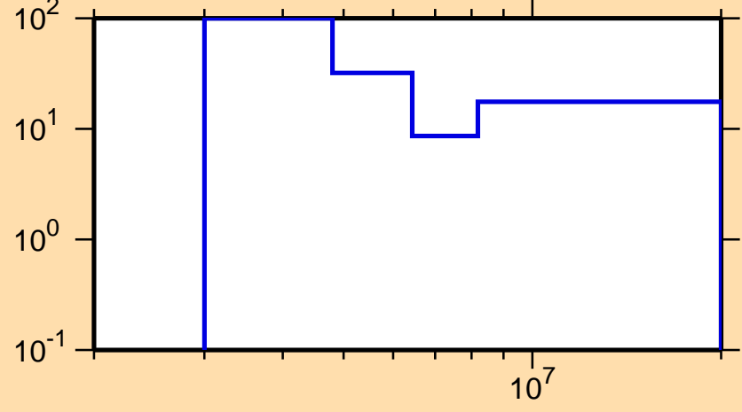
\Delta\sigma/\sigma vs. E for ^{211}\text{Po}(n,2n)
