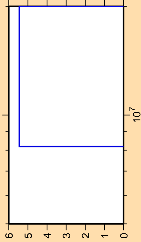
\Delta\sigma/\sigma vs. E for ^{211}\text{Po} (mt 42)
