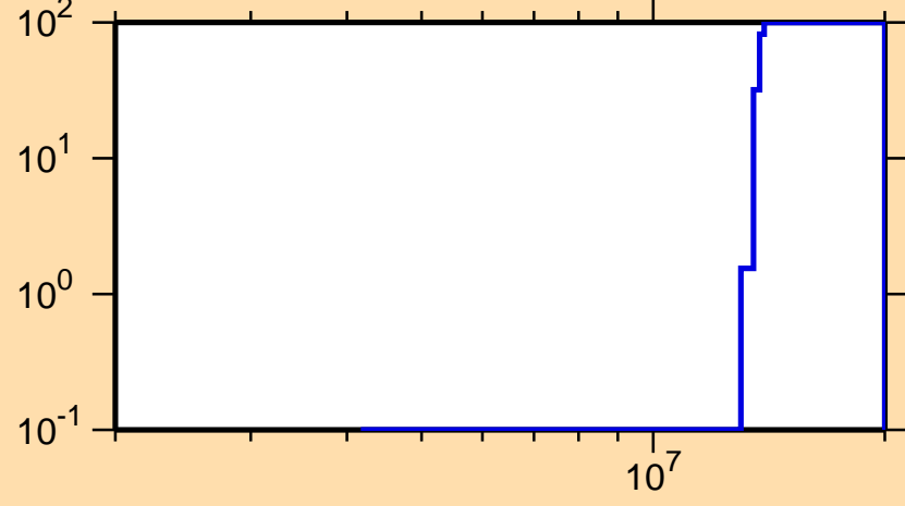
\Delta\sigma/\sigma vs. E for ^{217}\text{Po}(n,f)
