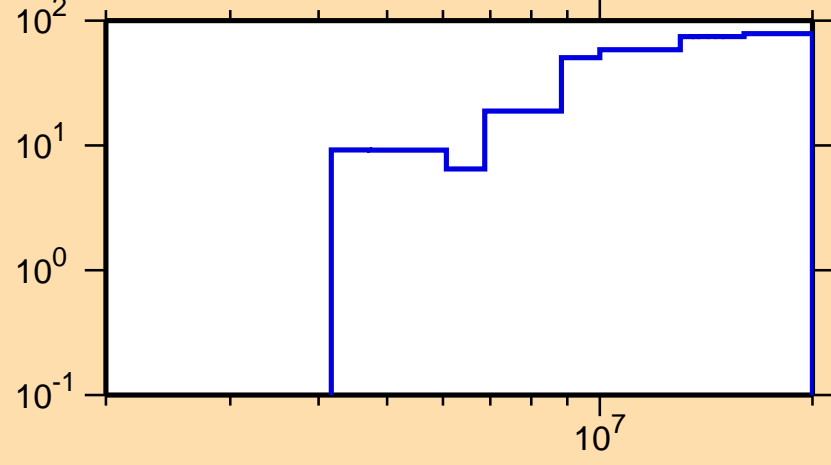
\Delta\sigma/\sigma vs. E for ^{217}\text{Po}(n,2n)
