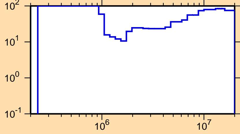
\Delta\sigma/\sigma vs. E for ^{217}\text{Po}(n,\text{inel.})
