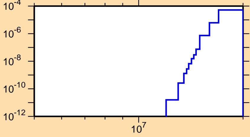
\sigma vs. E for ^{217}\text{Po}(n,\text{nt})
