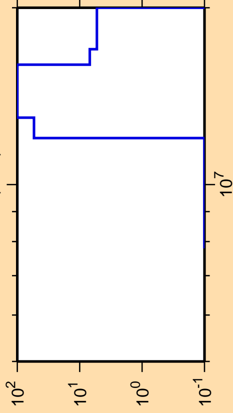
\Delta\sigma/\sigma vs. E for ^{217}\text{Po}(n,\text{nt})
