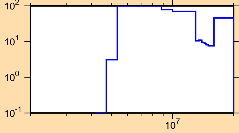
\Delta\sigma/\sigma vs. E for ^{217}\text{Po}(n,p)
