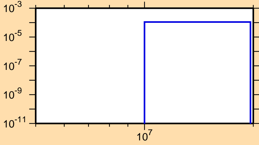
\sigma vs. E for ^{217}\text{Po}(n,d)
