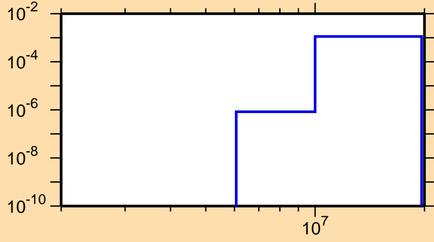
\sigma vs. E for ^{217}\text{Po}(n,p)
