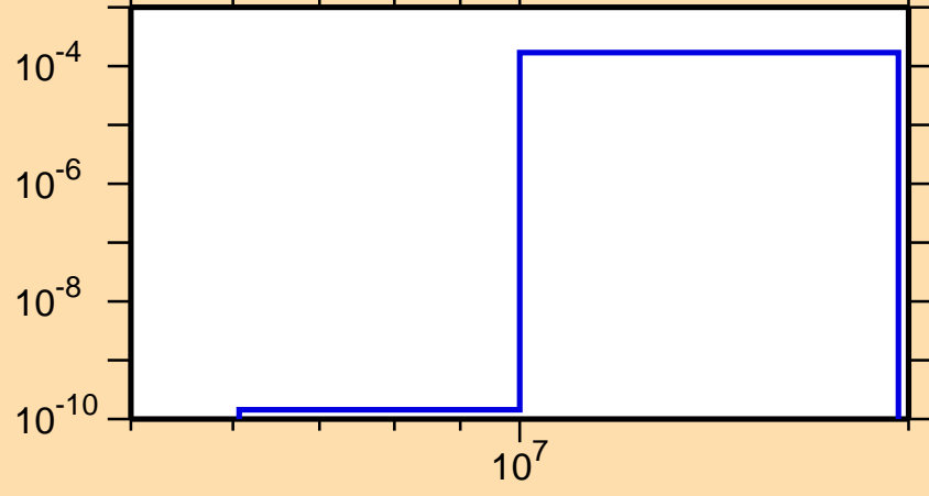
\sigma vs. E for ^{217}\text{Po}(n,t)
