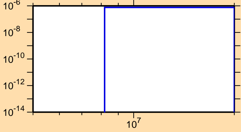
\sigma vs. E for ^{217}\text{Po}(n,nt)
