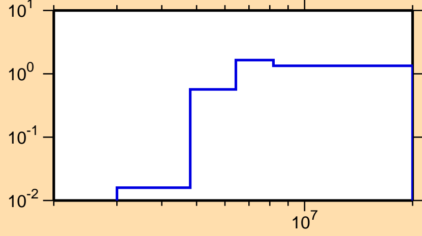
\sigma vs. E for ^{217}\text{Po}(n,2n)
