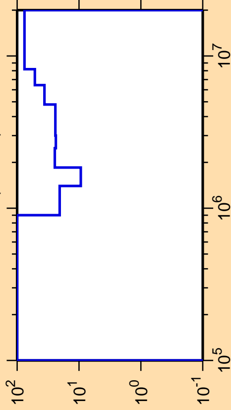
\Delta\sigma/\sigma vs. E for ^{217}\text{Po}(n,\text{inel.})
