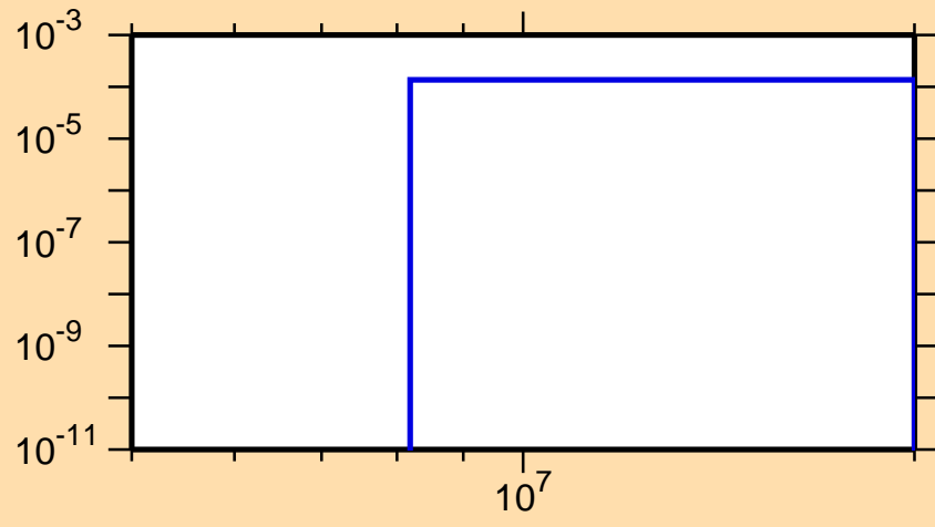
\sigma vs. E for ^{217}\text{Po}(n,t)
