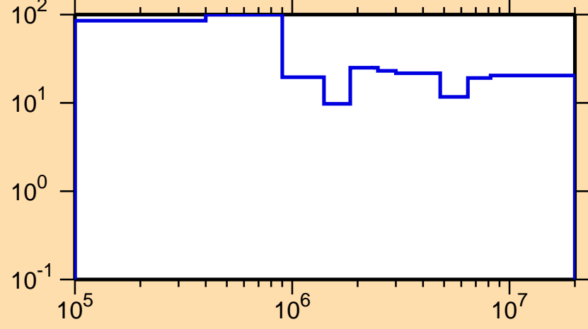
\Delta\sigma/\sigma vs. E for ^{217}\text{Po}(n,\text{nonel.})
