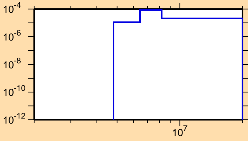
\sigma vs. E for ^{217}\text{Po}(n,2n\alpha)
