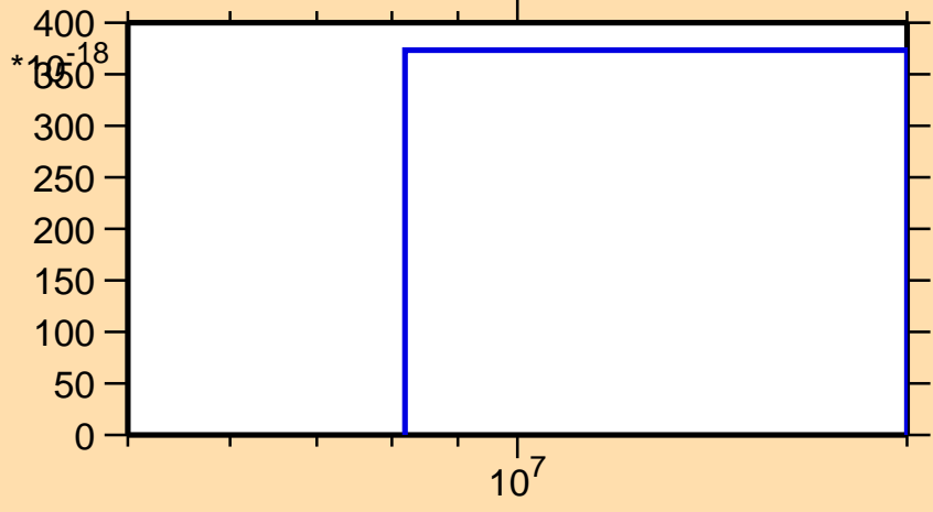
\sigma vs. E for ^{217}\text{Po} (mt 34)
