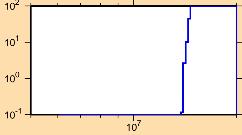
\Delta\sigma/\sigma vs. E for ^{218}\text{Po}(n,f)
