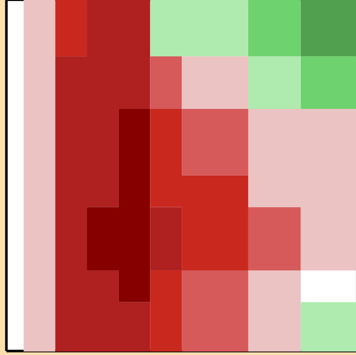
\Delta\sigma/\sigma vs. E for ^{218}\text{Po}(n,2n)
