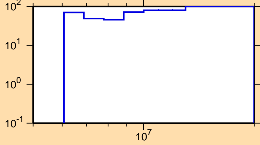
\Delta\sigma/\sigma vs. E for ^{218}\text{Po}(n,2n)
