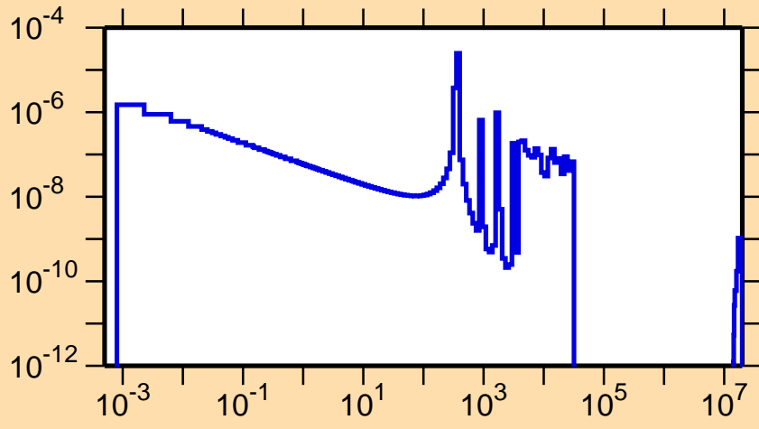
\sigma vs. E for ^{218}\text{Po}(n,f)
