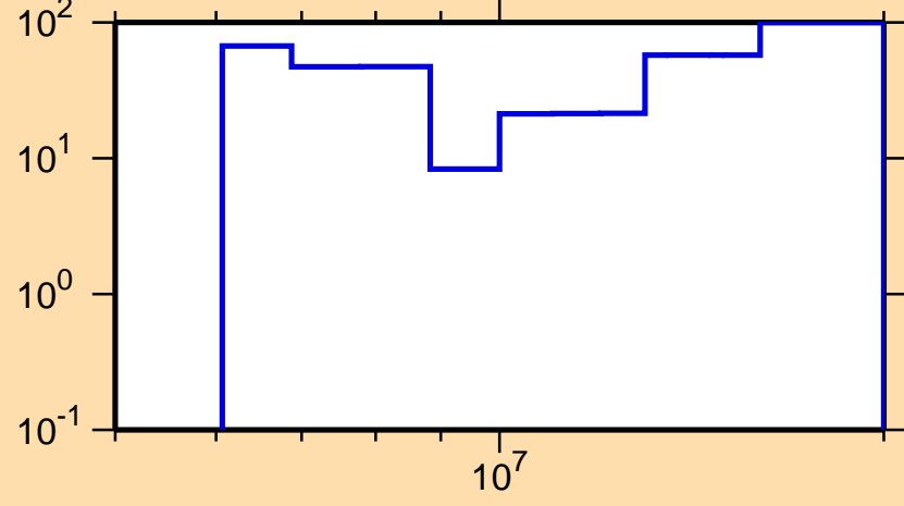
\Delta\sigma/\sigma vs. E for ^{218}\text{Po}(n,n\text{cont.})
