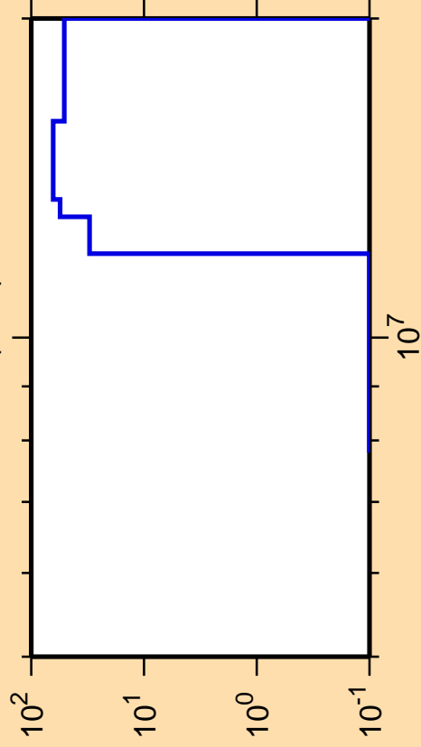
\Delta\sigma/\sigma vs. E for ^{218}\text{Po}(n,\text{nt})
