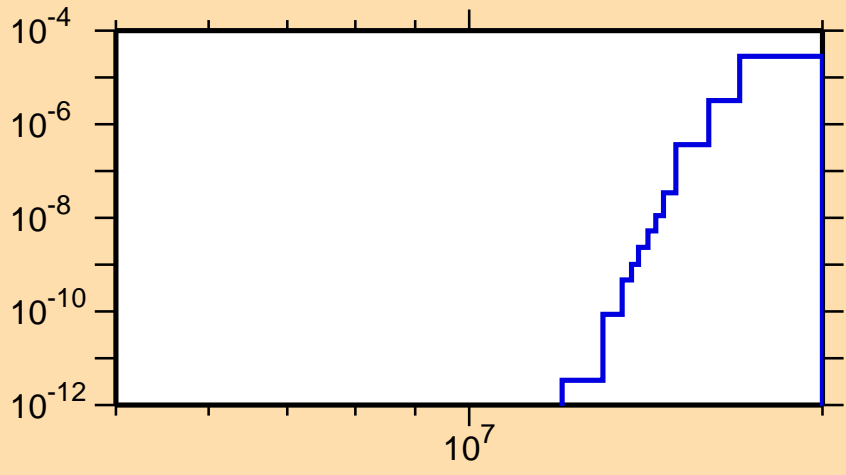
\sigma vs. E for ^{218}\text{Po}(n,\text{nt})
