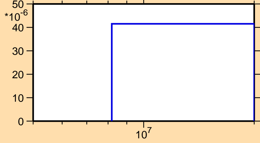
\sigma vs. E for ^{218}\text{Po}(n,t)
