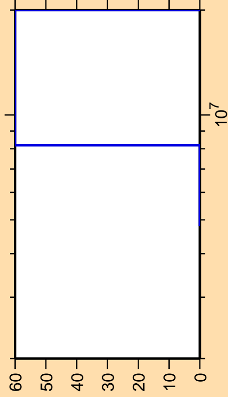
\Delta\sigma/\sigma vs. E for ^{218}\text{Po}(n,f)
