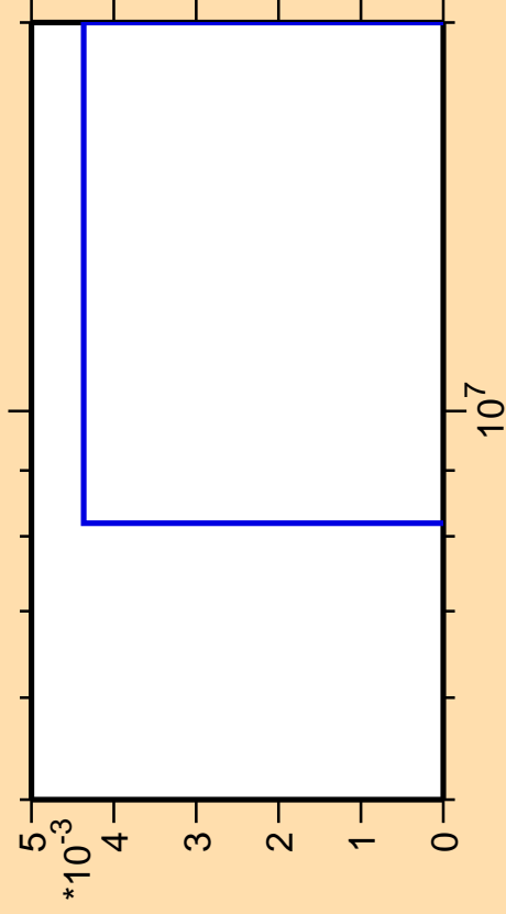
\Delta\sigma/\sigma vs. E for ^{218}\text{Po} (mt 42)
