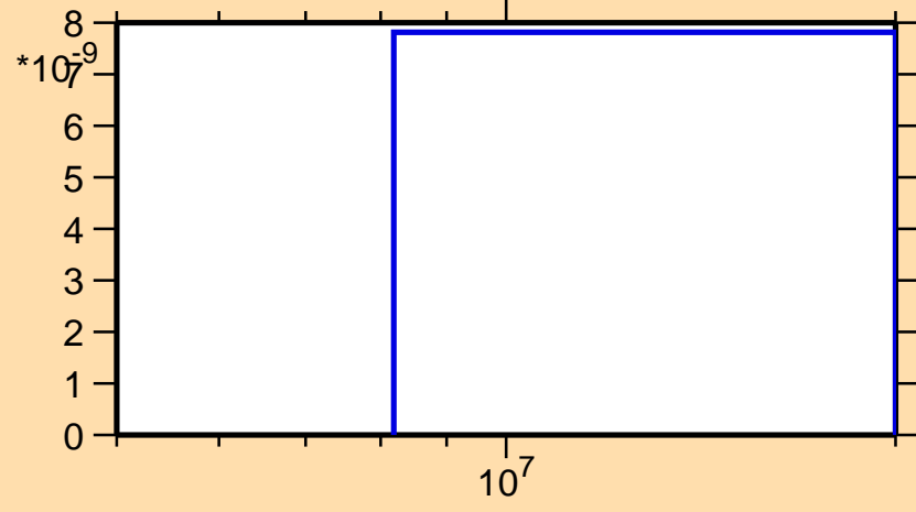
\sigma vs. E for ^{218}\text{Po}(n,\text{nd})
