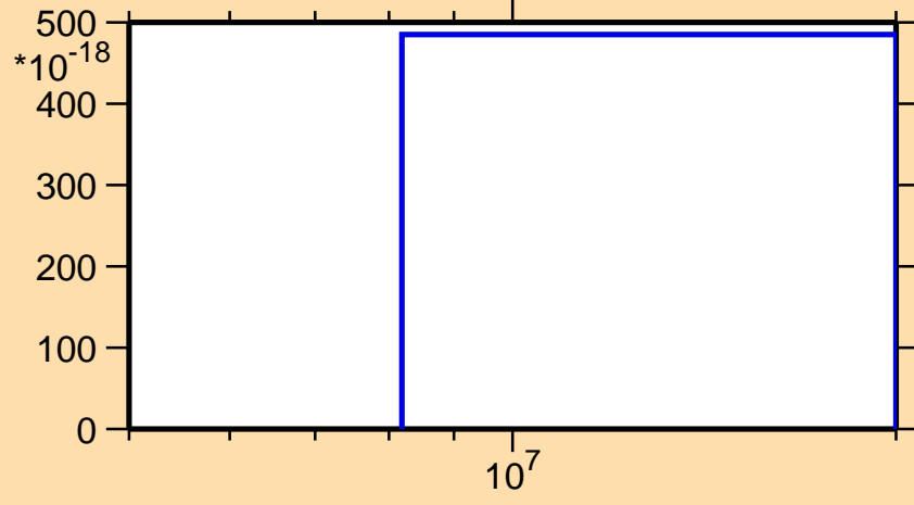
\sigma vs. E for ^{218}\text{Po} (mt 42)
