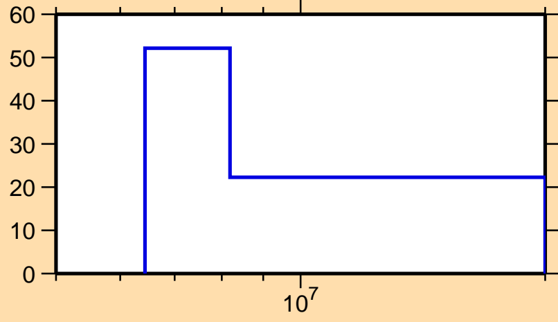
\Delta\sigma/\sigma vs. E for ^{218}\text{Po}(n,ncont.)
