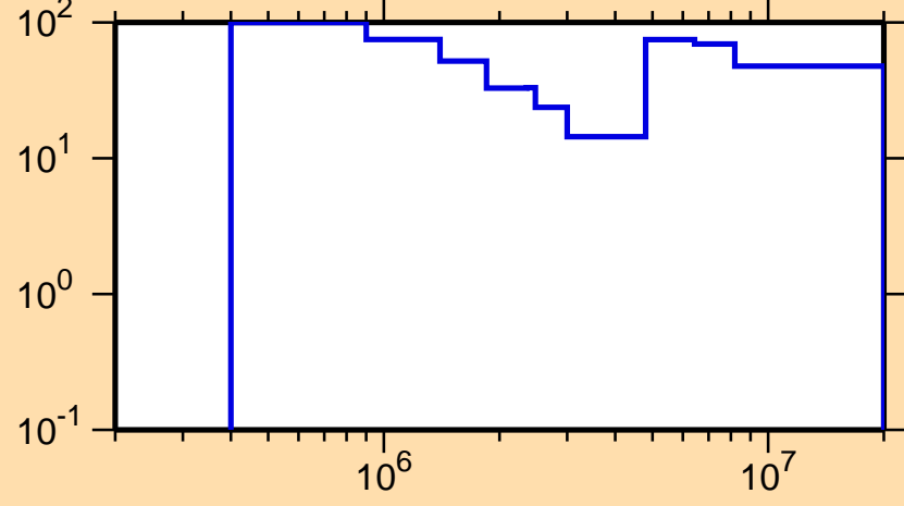
\Delta\sigma/\sigma vs. E for ^{218}\text{Po}(n,\text{inel.})
