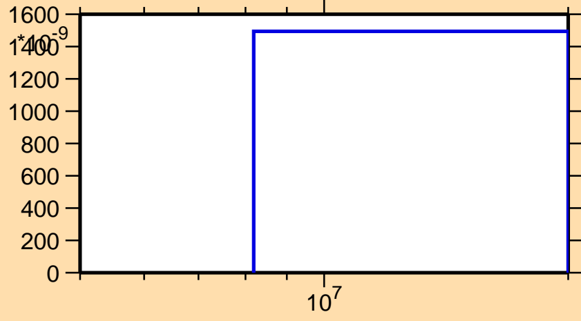
\sigma vs. E for ^{218}\text{Po}(n,3n\alpha)
