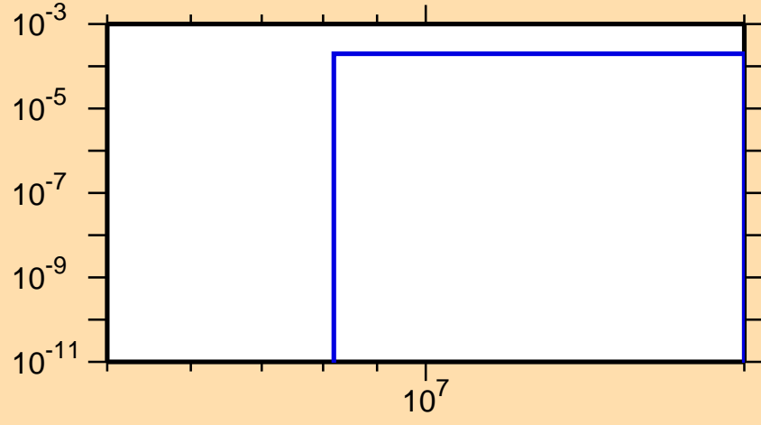
\sigma vs. E for ^{218}\text{Po}(n,p)
