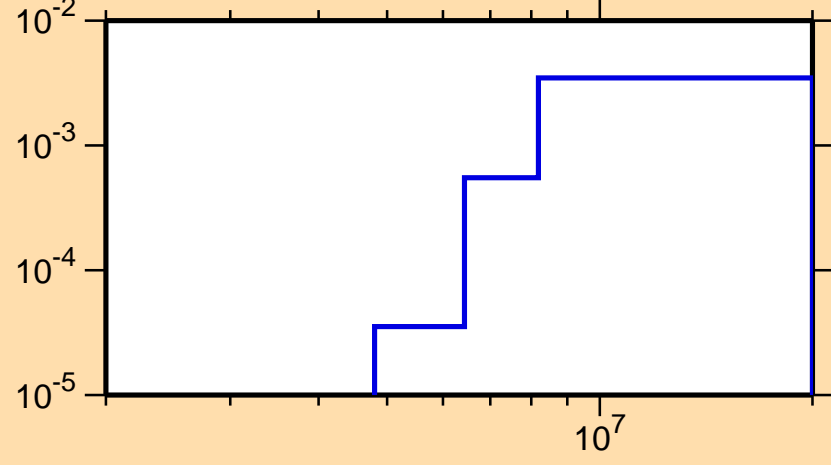
\sigma vs. E for ^{218}\text{Po}(n,2n\alpha)
