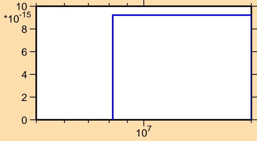
\sigma vs. E for ^{218}\text{Po}(n,\text{He3})
