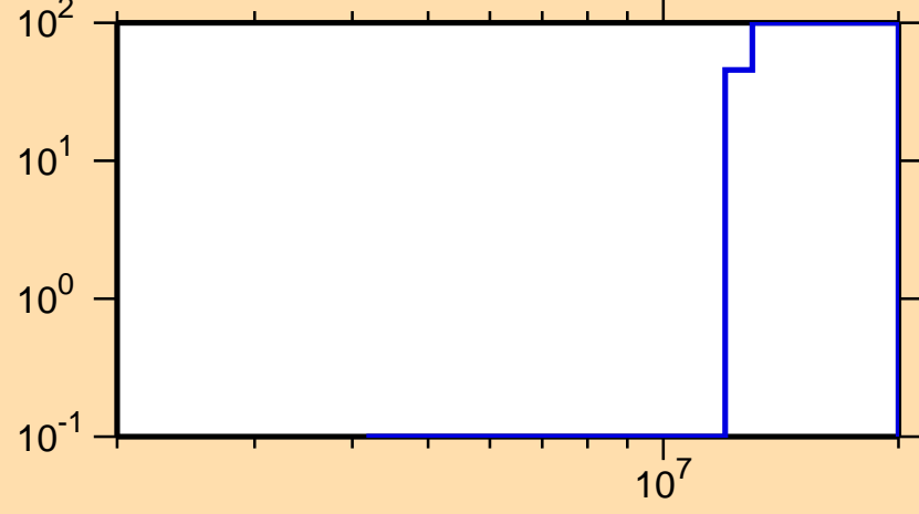
\Delta\sigma/\sigma vs. E for ^{219}\text{Po}(n,f)
