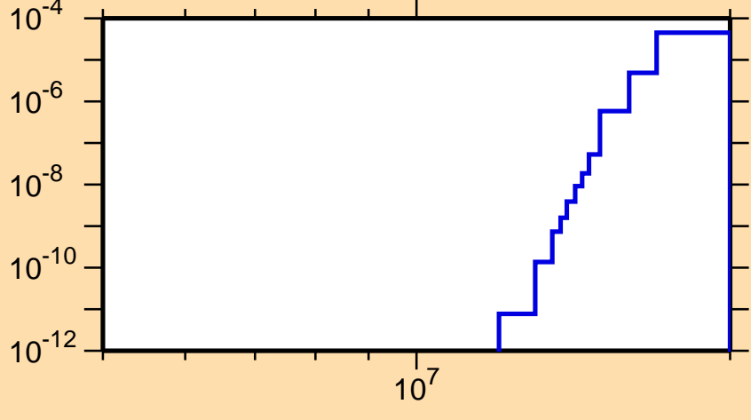
\sigma vs. E for ^{219}\text{Po}(n,\text{nt})
