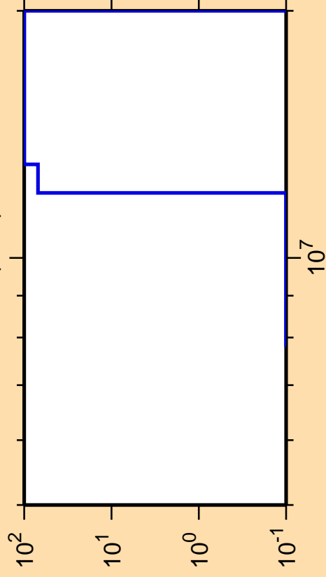
\Delta\sigma/\sigma vs. E for ^{219}\text{Po}(n,\text{nt})
