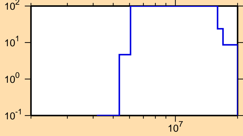
\Delta\sigma/\sigma vs. E for ^{219}\text{Po}(n,p)
