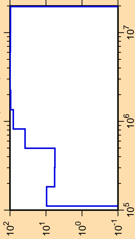
\Delta\sigma/\sigma vs. E for ^{219}\text{Po}(n,\text{inel.})
