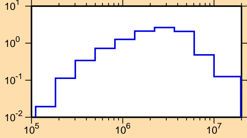
\sigma vs. E for ^{219}\text{Po}(n,n\text{cont.})
