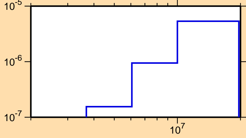
\sigma vs. E for ^{219}\text{Po}(n,2n\alpha)
