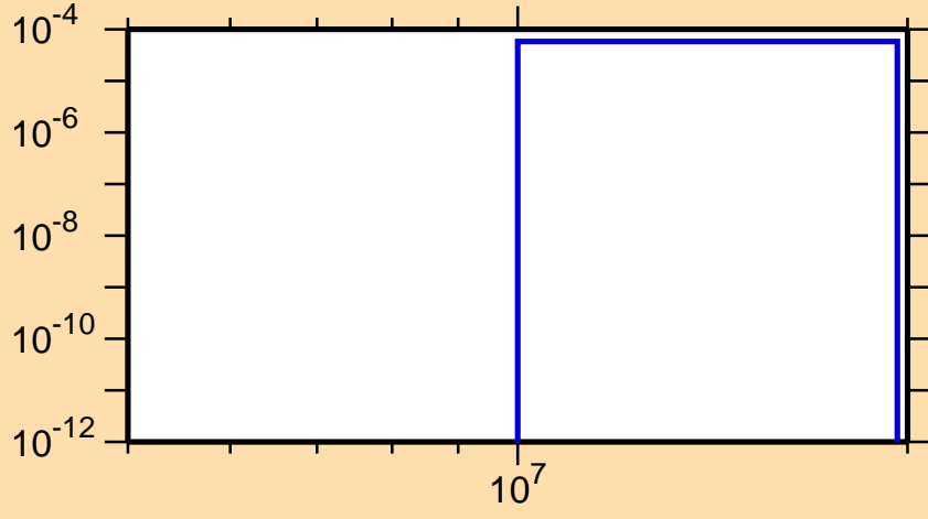
\sigma vs. E for ^{219}\text{Po}(n,d)
