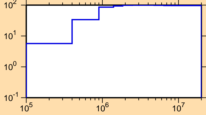
\Delta\sigma/\sigma vs. E for ^{219}\text{Po}(n,\text{inel.})
