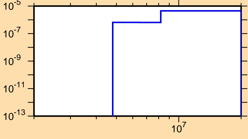
\sigma vs. E for ^{219}\text{Po}(n,2n\alpha)
