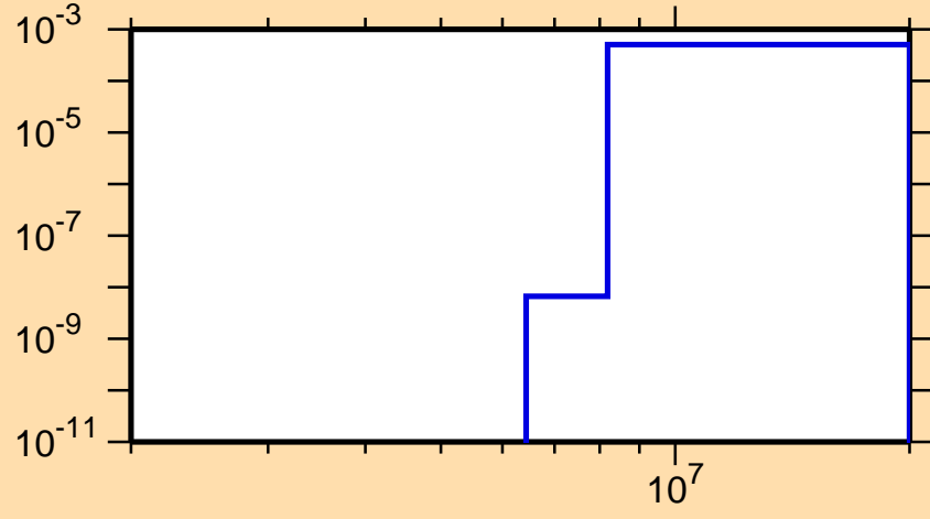
\sigma vs. E for ^{219}\text{Po}(n,p)
