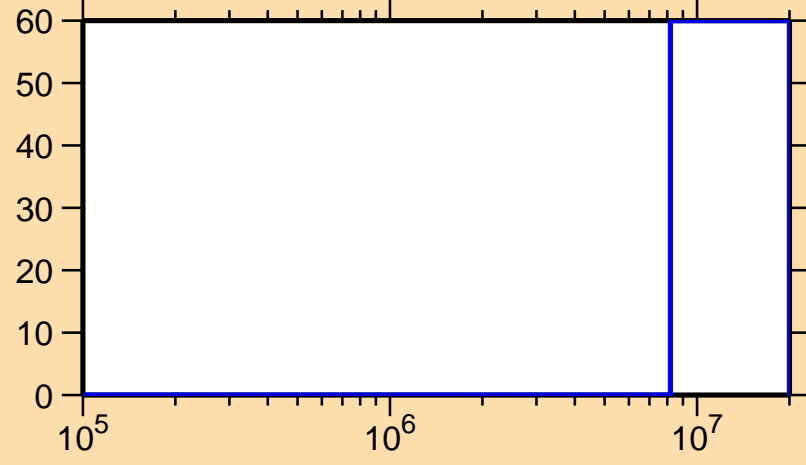
\Delta\sigma/\sigma vs. E for ^{219}\text{Po}(n,\text{f})
