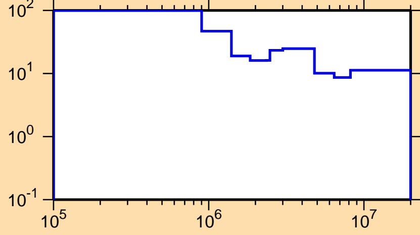
\Delta\sigma/\sigma vs. E for ^{219}\text{Po}(n,n\text{nonel.})
