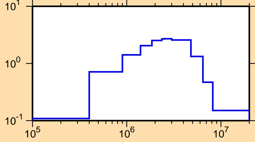
\sigma vs. E for ^{219}\text{Po}(n,\text{inel.})
