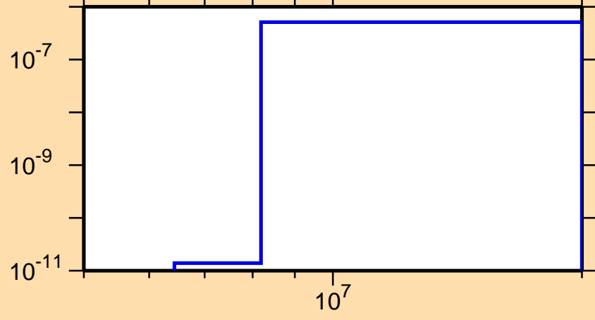
\sigma vs. E for ^{220}\text{Po}(n,2n\alpha)
