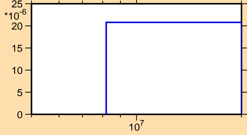
\sigma vs. E for ^{220}\text{Po}(n,t)
