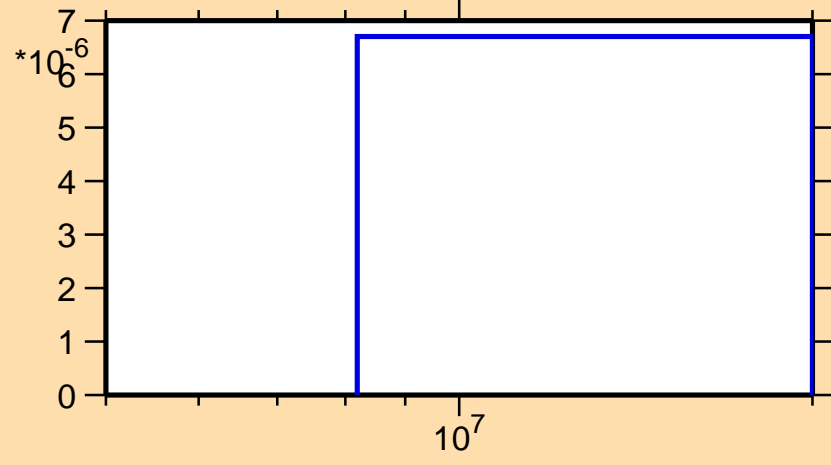
\sigma vs. E for ^{220}\text{Po}(n,np)
