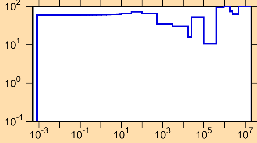
\Delta\sigma/\sigma vs. E for ^{220}\text{Po}(n,\text{el.})
