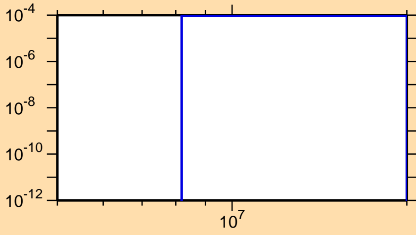
\sigma vs. E for ^{220}\text{Po}(n,p)
