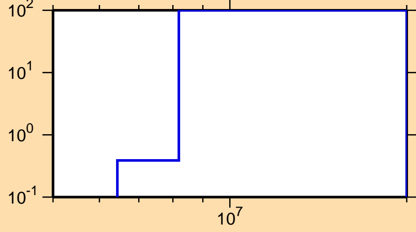
\Delta\sigma/\sigma vs. E for ^{220}\text{Po}(n,p)
