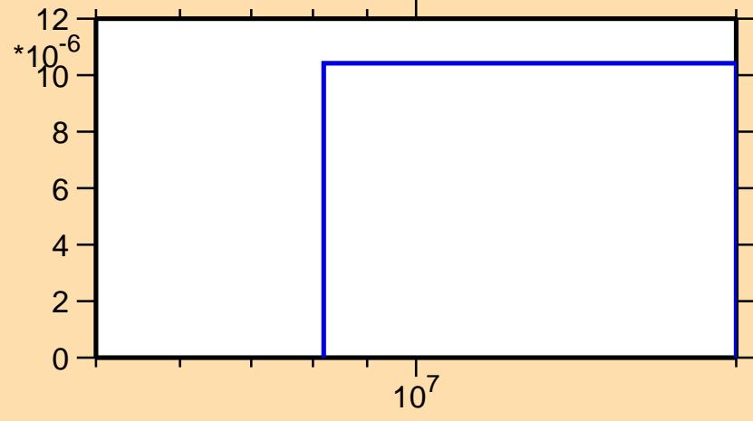
\sigma vs. E for ^{220}\text{Po}(n,d)
