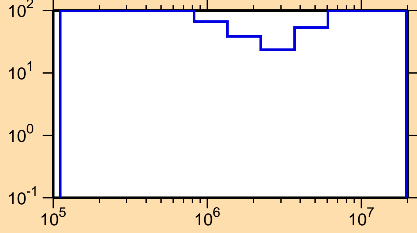
\Delta\sigma/\sigma vs. E for ^{221}\text{Po}(n,\text{inel.})
