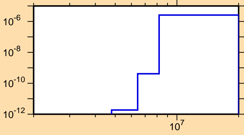
\sigma vs. E for ^{221}\text{Po}(n,2n\alpha)
