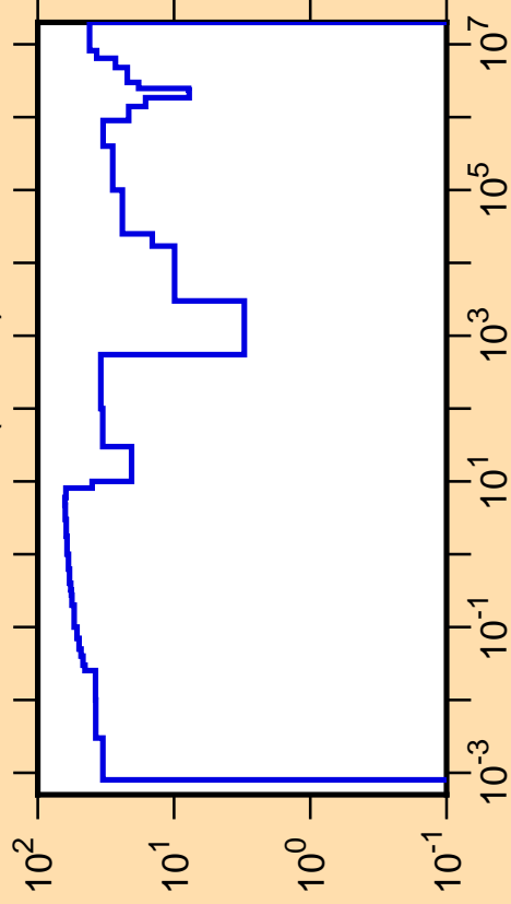
\Delta\sigma/\sigma vs. E for ^{221}\text{Po}(n,\text{tot.})
