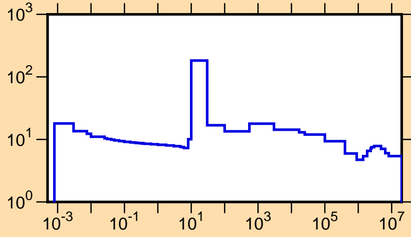
\sigma vs. E for ^{221}\text{Po}(n,\text{tot.})
