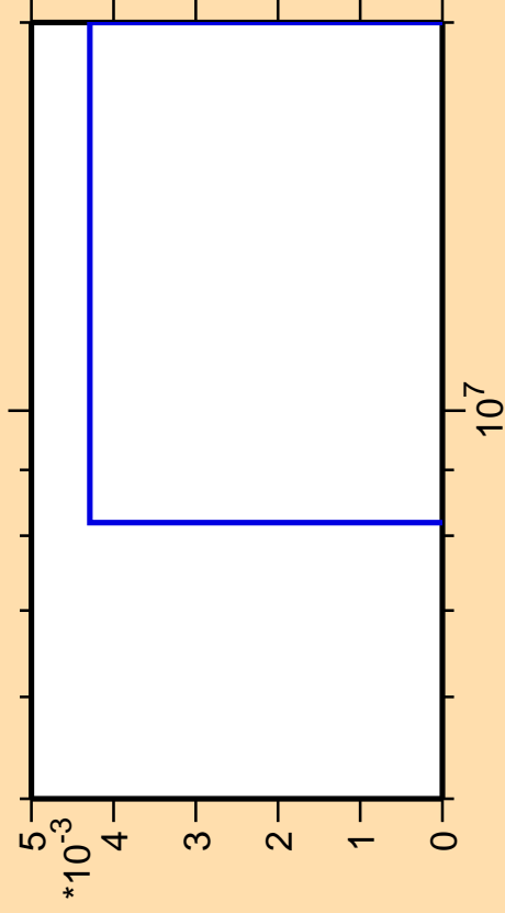
\Delta\sigma/\sigma vs. E for ^{221}\text{Po} (mt 42)
