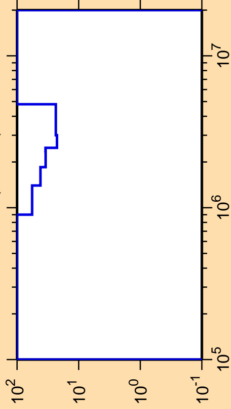
\Delta\sigma/\sigma vs. E for ^{221}\text{Po}(n,\text{inel.})
