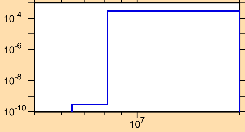
\sigma vs. E for ^{221}\text{Po}(n,p)
