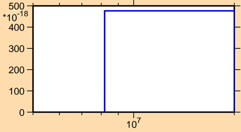
\sigma vs. E for ^{221}\text{Po} (mt 42)
