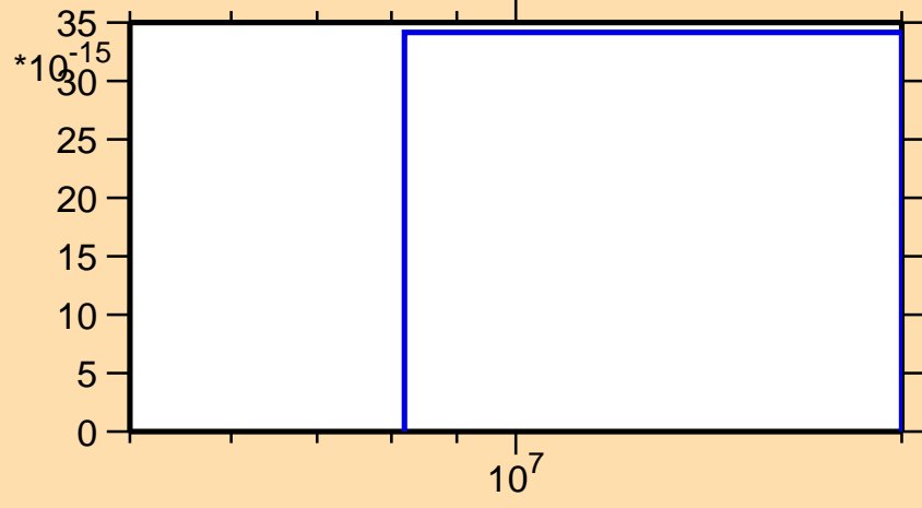
\sigma vs. E for ^{221}\text{Po} (mt 11)
