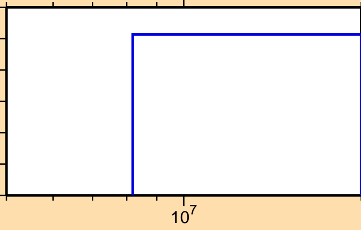
\sigma vs. E for ^{221}\text{Po}(n,t)
