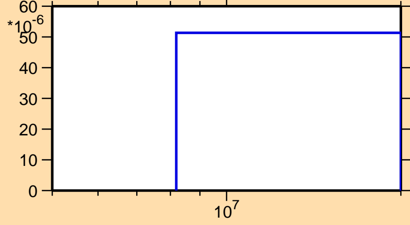
\sigma vs. E for ^{221}\text{Po}(n,t)
