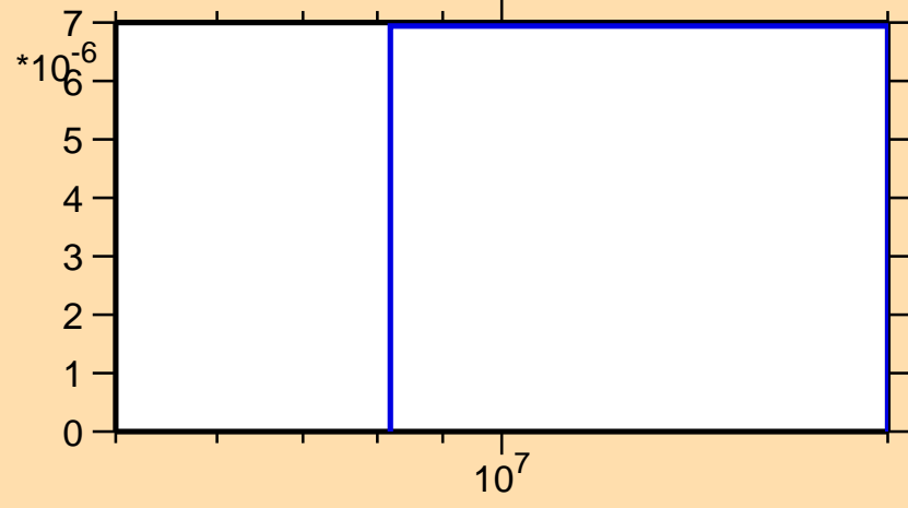
\sigma vs. E for ^{221}\text{Po}(n,np)
