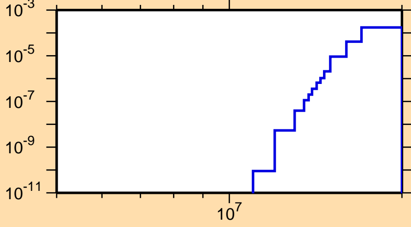
\sigma vs. E for ^{222}\text{Po}(n,d)
