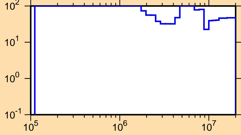
\Delta\sigma/\sigma vs. E for ^{222}\text{Po}(n,\text{inel.})
