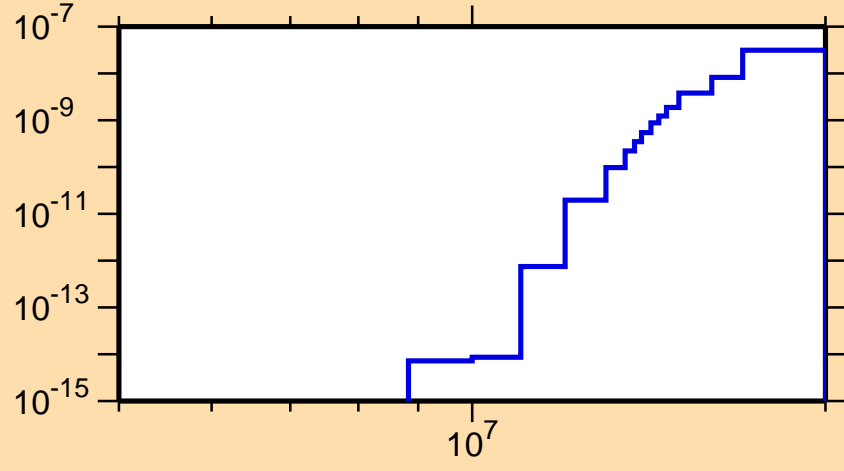
\sigma vs. E for ^{222}\text{Po}(n,3n\alpha)
