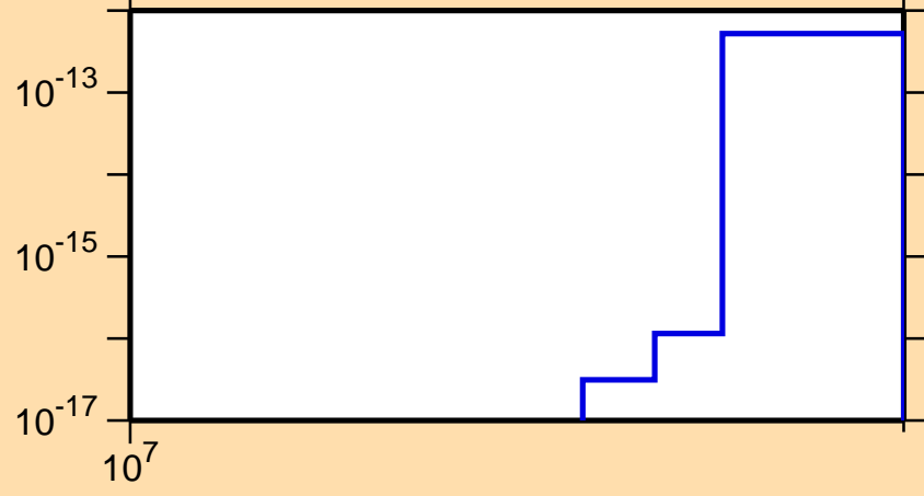
\sigma vs. E for ^{222}\text{Po} (mt 11)
