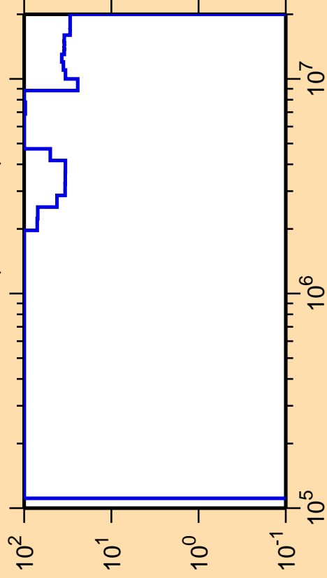
\Delta\sigma/\sigma vs. E for ^{222}\text{Po}(n,\text{ncont.})
