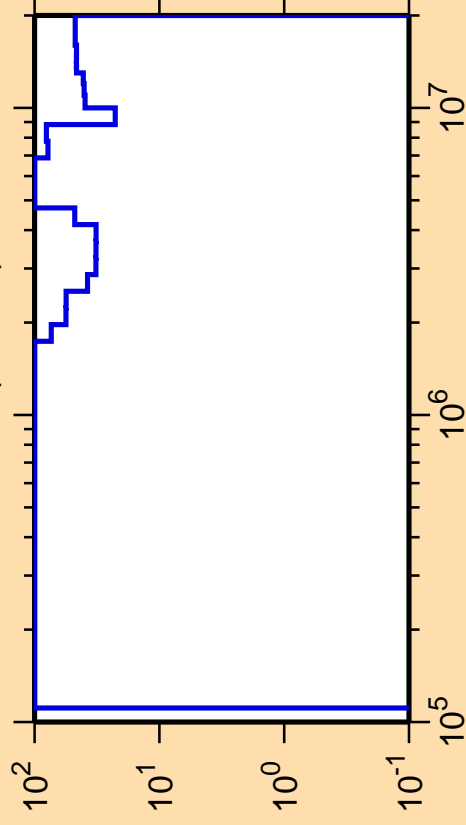
\Delta\sigma/\sigma vs. E for ^{222}\text{Po}(n,\text{inel.})
