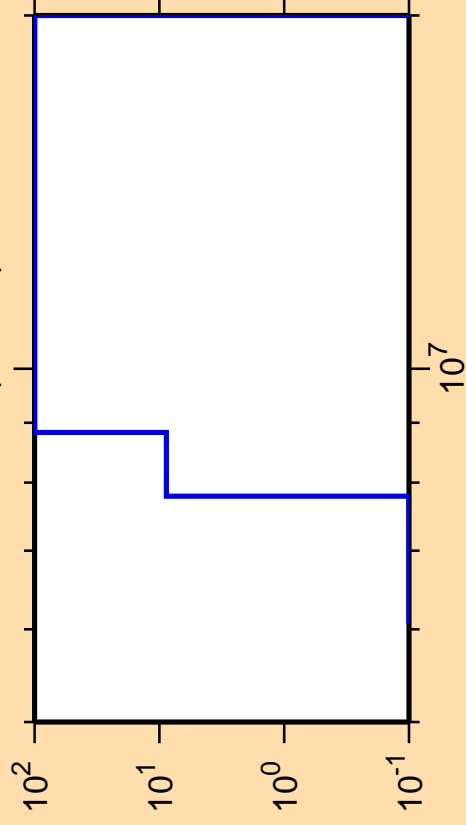
\Delta\sigma/\sigma vs. E for ^{222}\text{Po}(n,2n\alpha)
