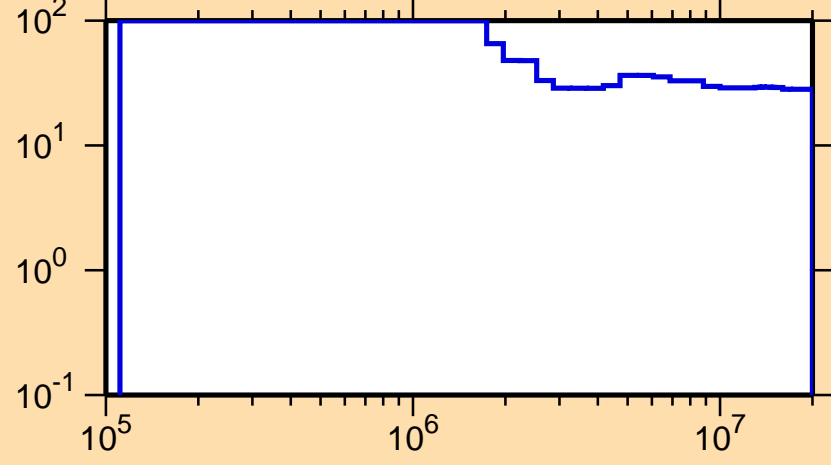
\Delta\sigma/\sigma vs. E for ^{222}\text{Po}(n,\text{nonel.})
