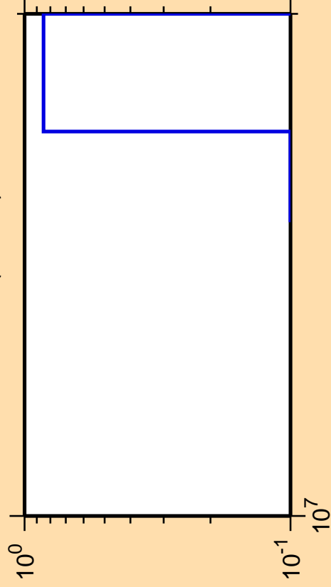
\Delta\sigma/\sigma vs. E for ^{222}\text{Po} (mt 11)
