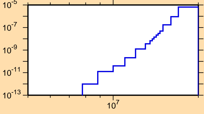
\sigma vs. E for ^{222}\text{Po}(n,2n\alpha)
