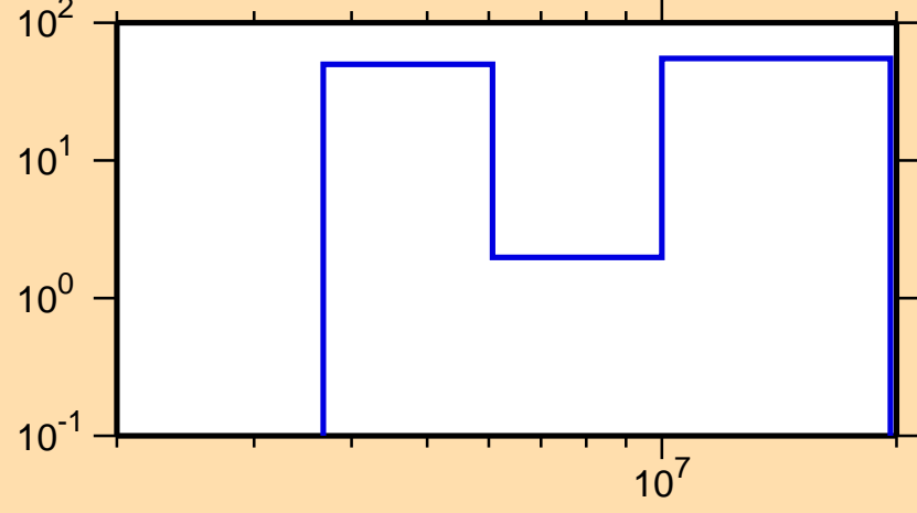
\Delta\sigma/\sigma vs. E for ^{222}\text{Po}(n,2n)
