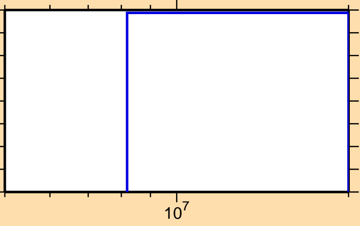
\sigma vs. E for ^{222}\text{Po}(n,nt)
