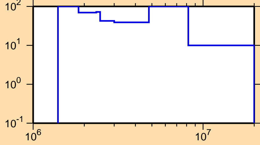
\Delta\sigma/\sigma vs. E for ^{222}\text{Po}(n,n\text{cont.})
