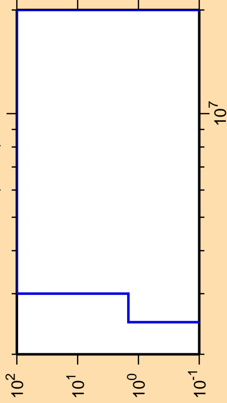
\Delta\sigma/\sigma vs. E for ^{222}\text{Po}(n,n\alpha)
