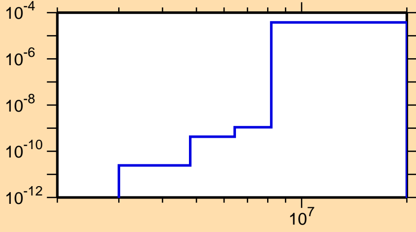
\sigma vs. E for ^{222}\text{Po}(n,n\alpha)
