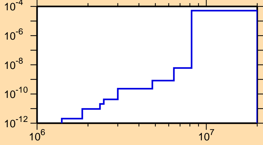
\sigma vs. E for ^{222}\text{Po}(n,\alpha)
