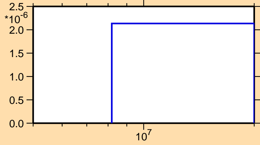
\sigma vs. E for ^{222}\text{Po}(n,np)
