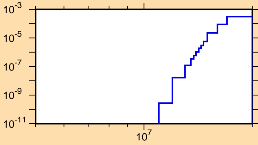
\sigma vs. E for ^{223}\text{Po}(n,d)
