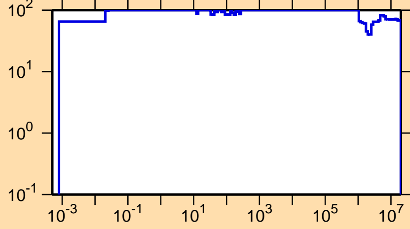
\Delta\sigma/\sigma vs. E for ^{223}\text{Po}(n,\text{nonel.})
