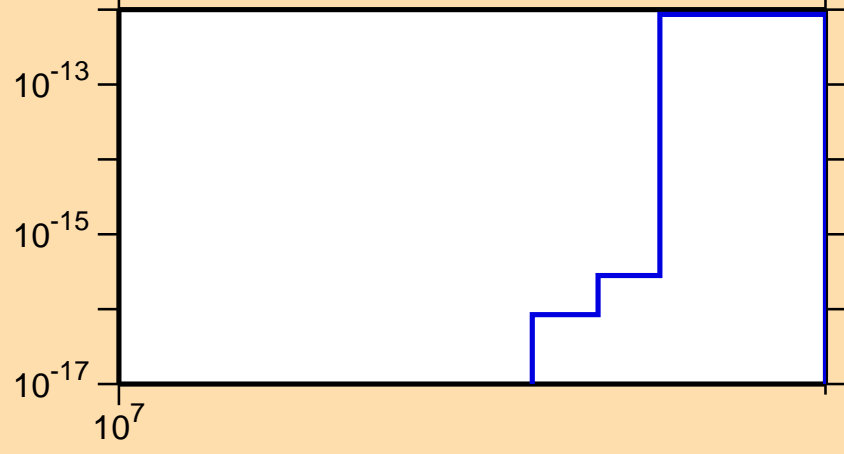
\sigma vs. E for ^{223}\text{Po} (mt 11)
