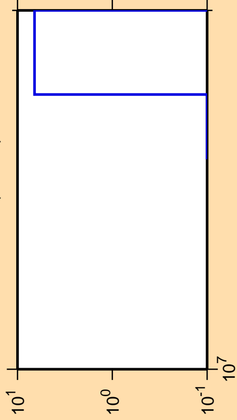
\Delta\sigma/\sigma vs. E for ^{223}\text{Po} (mt 11)
