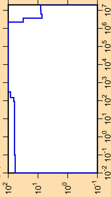
\Delta\mu/\mu vs. E for ^{223}\text{Po}(\text{mt251})
