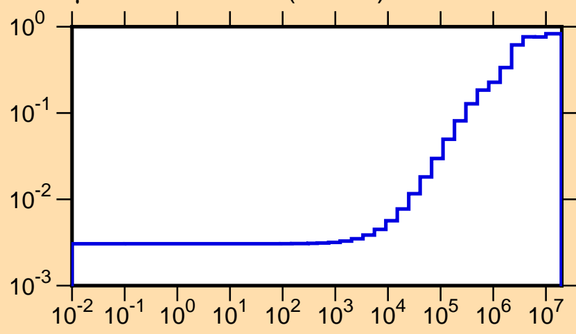
\mu vs. E for ^{223}\text{Po}(\text{mt251})
