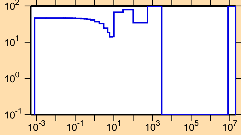
\Delta\sigma/\sigma vs. E for ^{223}\text{Po}(n,f)
