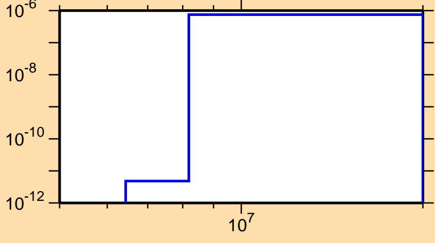
\sigma vs. E for ^{223}\text{Po}(n,2n\alpha)
