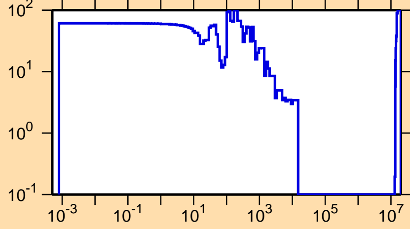
\Delta\sigma/\sigma vs. E for ^{224}\text{Po}(n,f)
