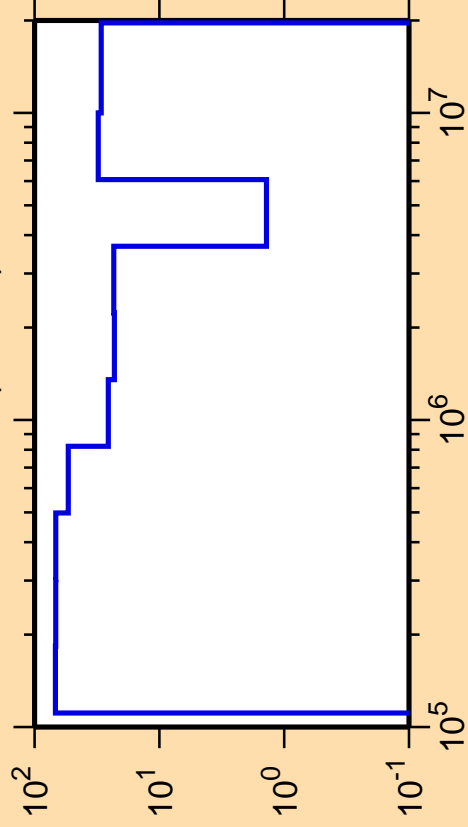
\Delta\sigma/\sigma vs. E for ^{224}\text{Po}(n,\text{inel.})
