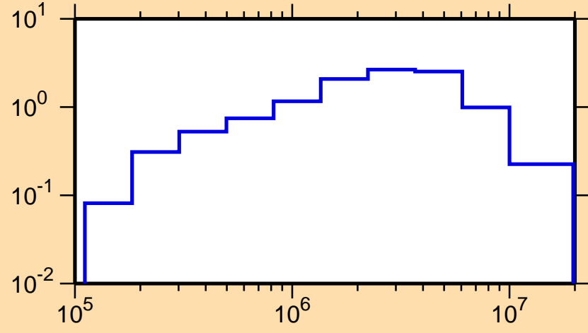
\sigma vs. E for ^{224}\text{Po}(n,\text{inel.})
