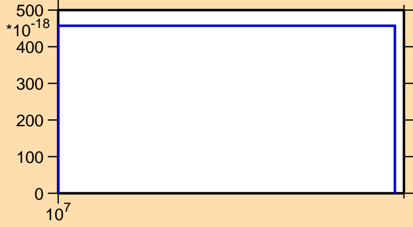
\sigma vs. E for ^{224}\text{Po} (mt 11)
