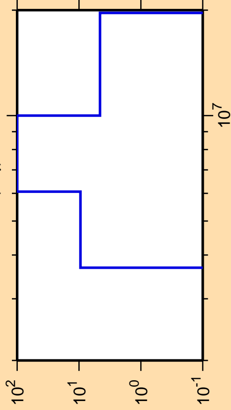
\Delta\sigma/\sigma vs. E for ^{224}\text{Po}(n,\gamma)
