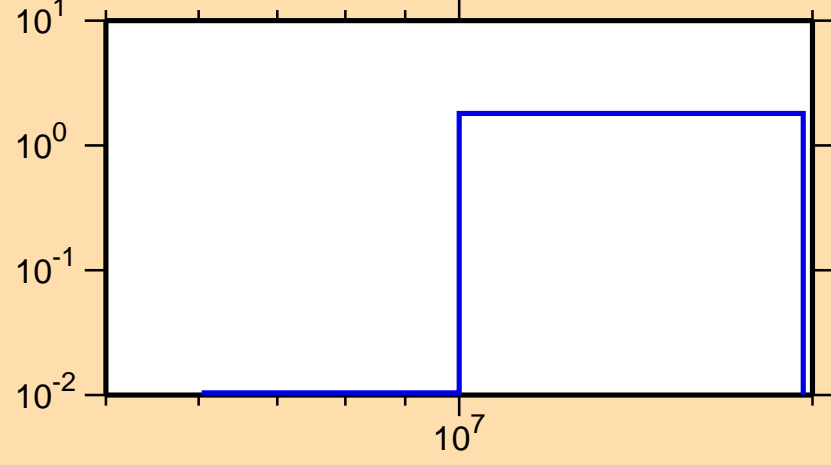
\sigma vs. E for ^{224}\text{Po}(n,3n)
