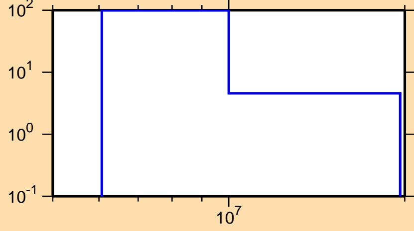
\Delta\sigma/\sigma vs. E for ^{224}\text{Po}(n,\gamma)
