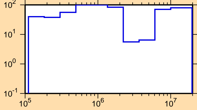
\Delta\sigma/\sigma vs. E for ^{224}\text{Po}(n,\text{el.})
