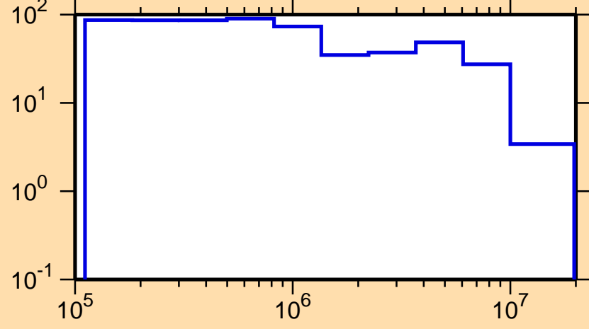
\Delta\sigma/\sigma vs. E for ^{224}\text{Po}(n,n_1)
