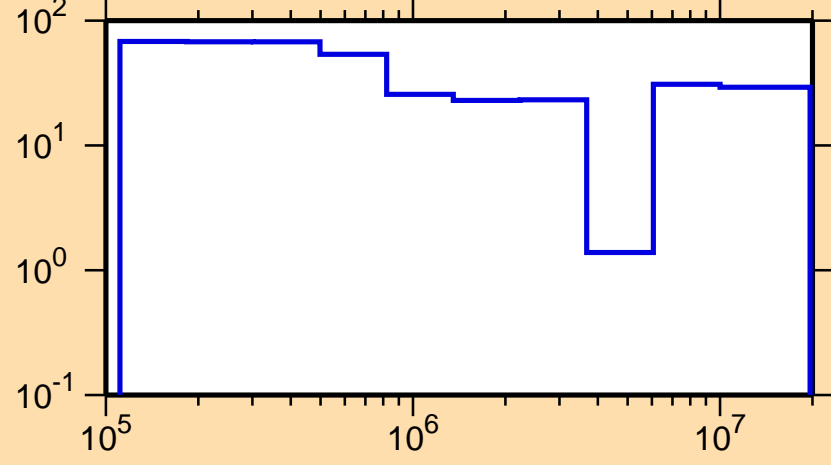
\Delta\sigma/\sigma vs. E for ^{224}\text{Po}(n,\text{inel.})
