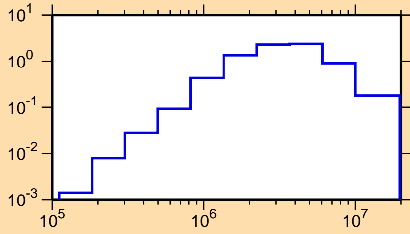
\sigma vs. E for ^{224}\text{Po}(n,n\text{cont.})
