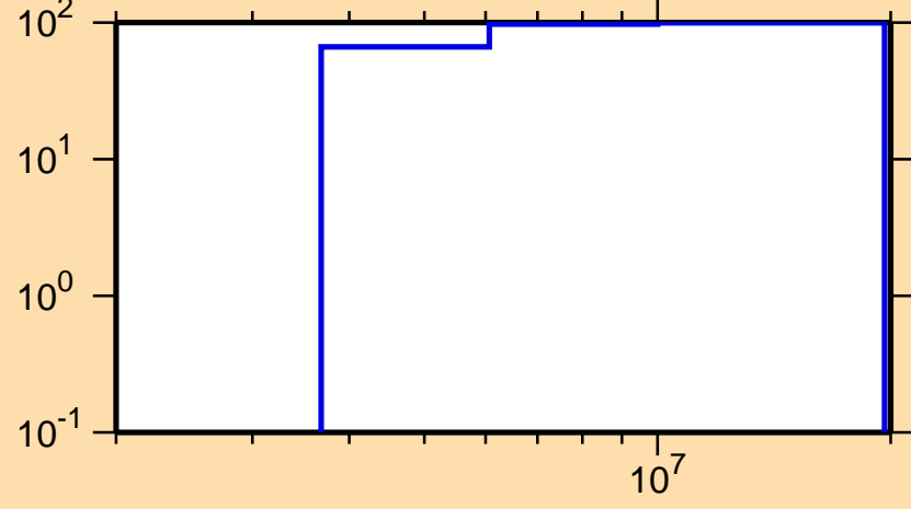
\Delta\sigma/\sigma vs. E for ^{224}\text{Po}(n,2n)
