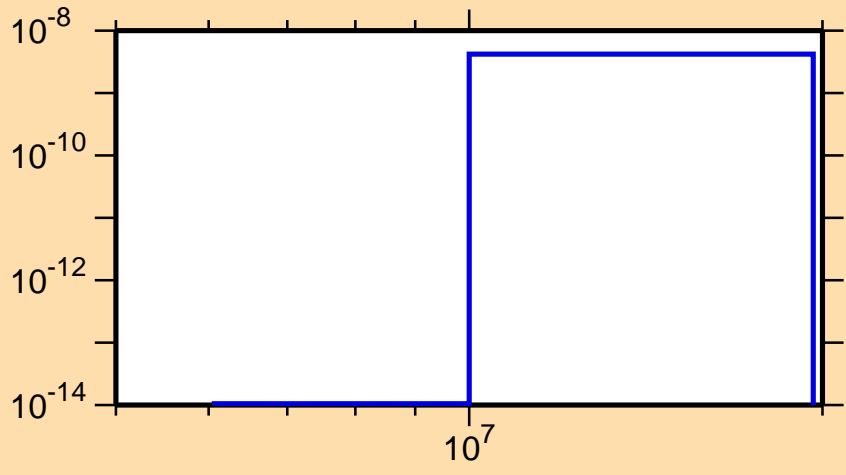
\sigma vs. E for ^{224}\text{Po}(n,2n\alpha)
