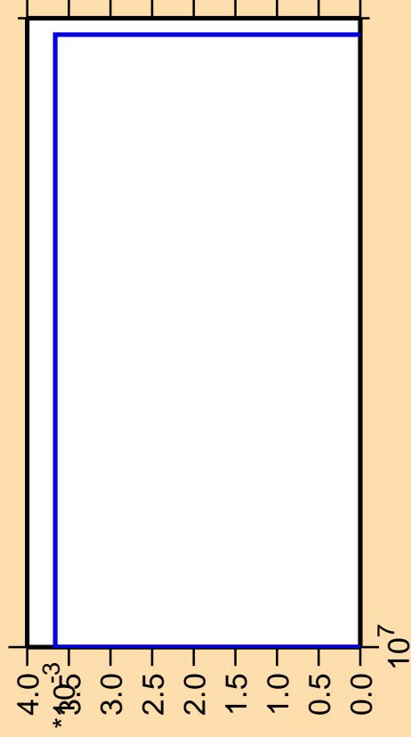
\Delta\sigma/\sigma vs. E for ^{224}\text{Po} (mt 11)
