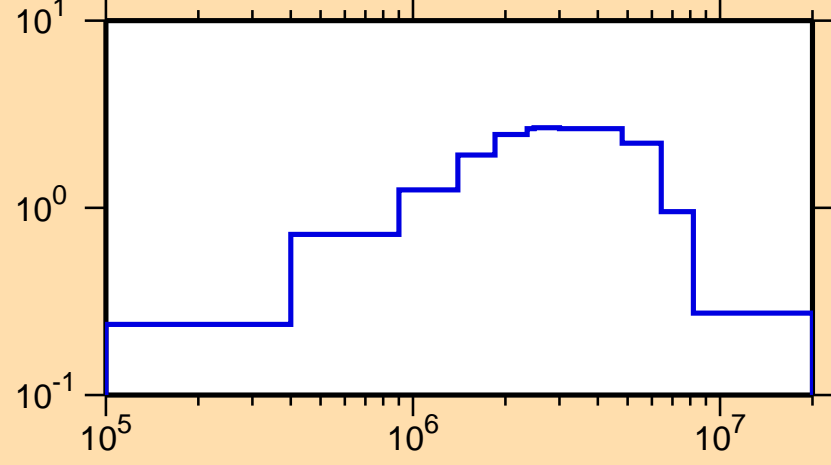
\sigma vs. E for ^{224}\text{Po}(n,\text{inel.})
