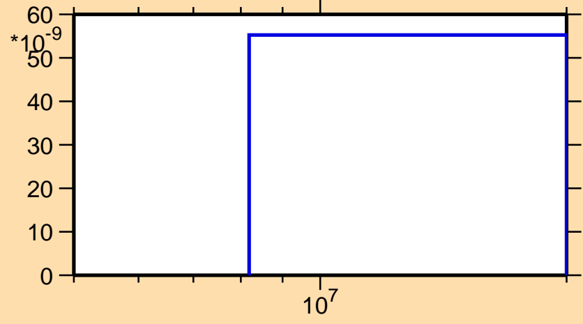
\sigma vs. E for ^{224}\text{Po}(n,\text{nt})
