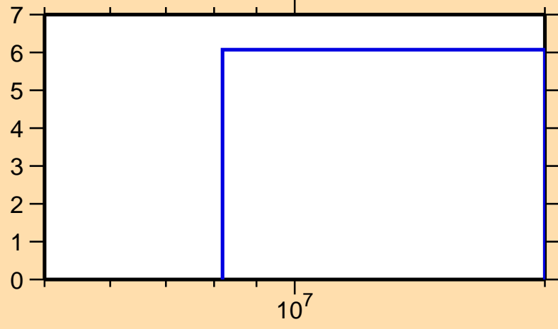
\Delta\sigma/\sigma vs. E for ^{224}\text{Po}(n,n_1)
