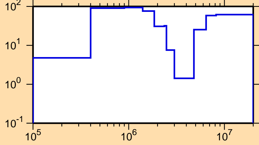
\Delta\sigma/\sigma vs. E for ^{224}\text{Po}(n,\text{tot.})
