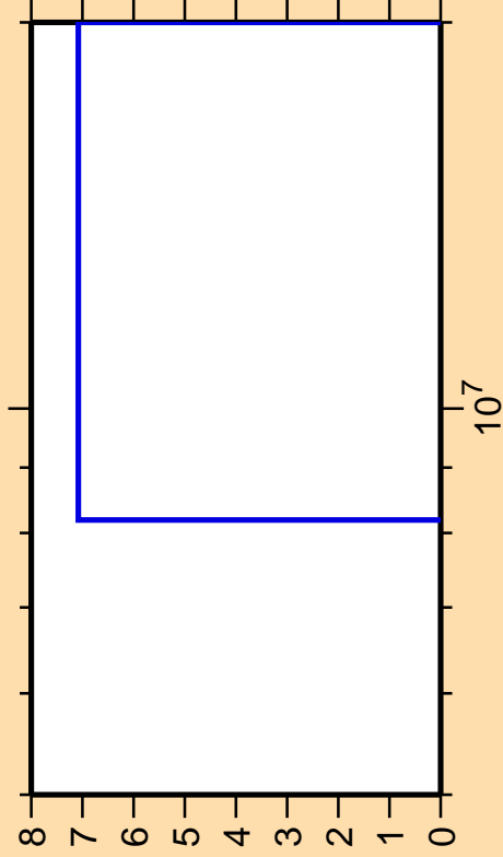
\Delta\sigma/\sigma vs. E for ^{224}\text{Po}(n,d)
