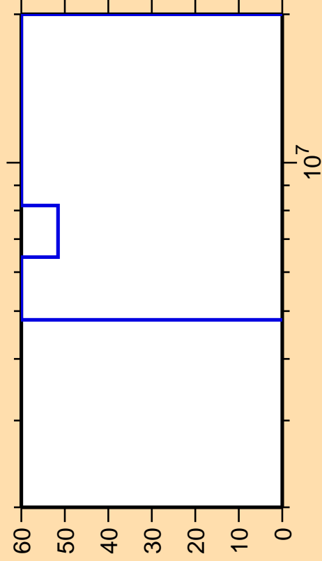
\Delta\sigma/\sigma vs. E for ^{224}\text{Po}(n,2n)
