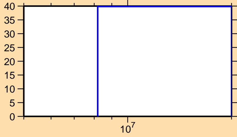
\Delta\sigma/\sigma vs. E for ^{224}\text{Po}(n,ncont.)
