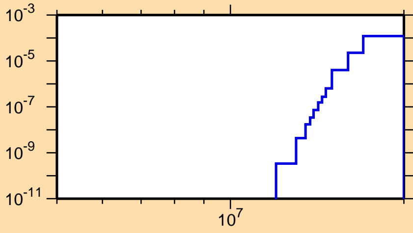
\sigma vs. E for ^{225}\text{Po}(n,d)
