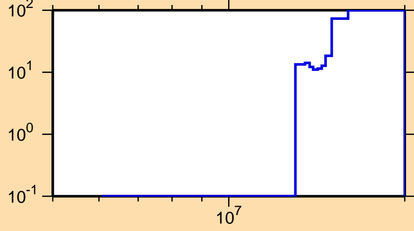
\Delta\sigma/\sigma vs. E for ^{225}\text{Po}(n,f)
