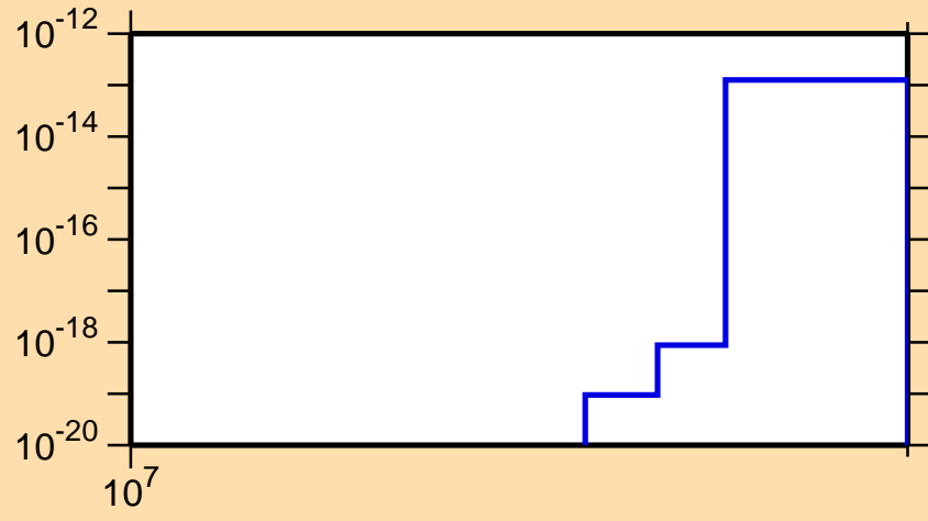
\sigma vs. E for ^{225}\text{Po}(\text{mt 11})
