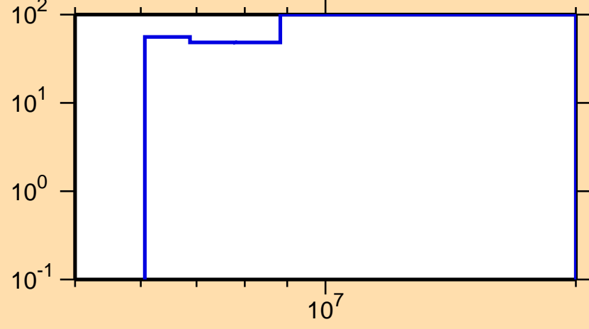
\Delta\sigma/\sigma vs. E for ^{225}\text{Po}(n,2n)
