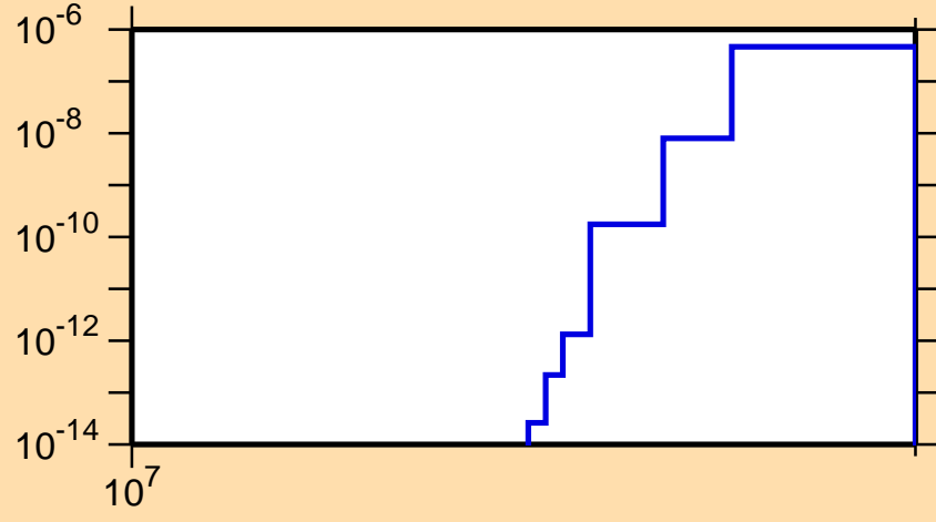
\sigma vs. E for ^{225}\text{Po}(n,\text{nd})
