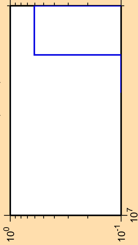
\Delta\sigma/\sigma vs. E for ^{225}\text{Po}(\text{mt 11})
