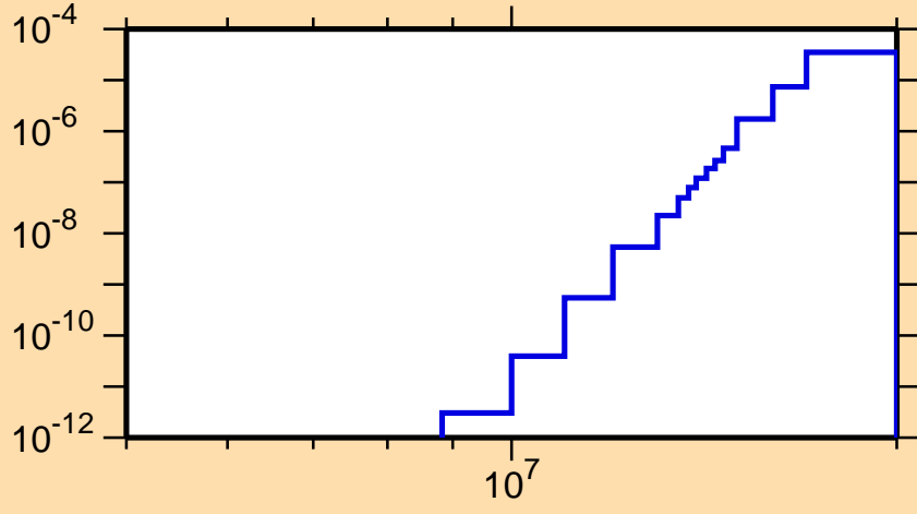
\sigma vs. E for ^{225}\text{Po}(n,n\alpha)
