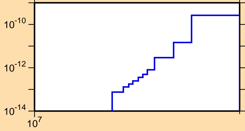
\sigma vs. E for ^{225}\text{Po}(n,3n\alpha)
