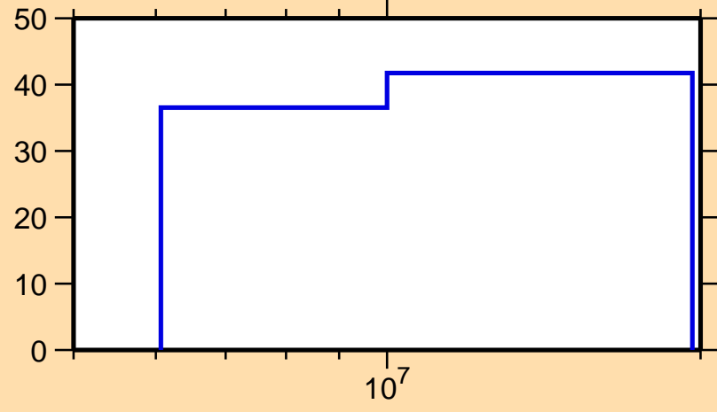
\Delta\sigma/\sigma vs. E for ^{225}\text{Po}(n,ncont.)
