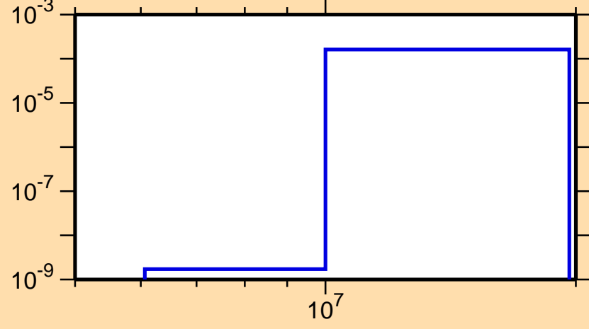
\sigma vs. E for ^{225}\text{Po}(n,p)
