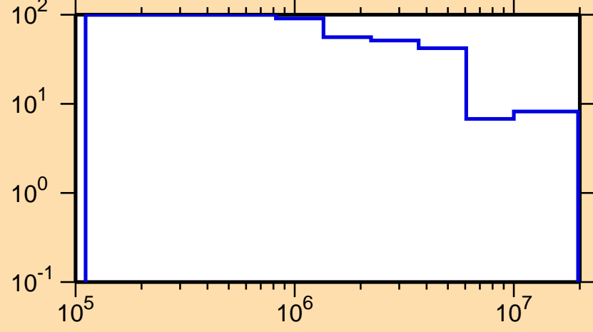
\Delta\sigma/\sigma vs. E for ^{225}\text{Po}(n,\text{inel.})
