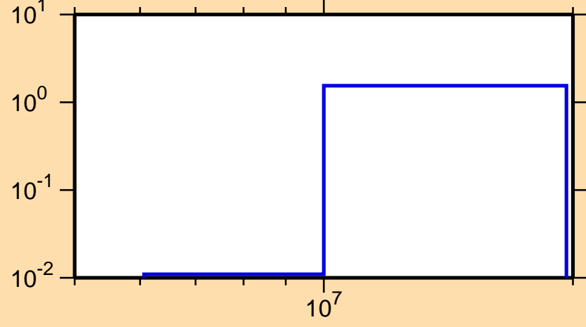
\sigma vs. E for ^{225}\text{Po}(n,3n)
