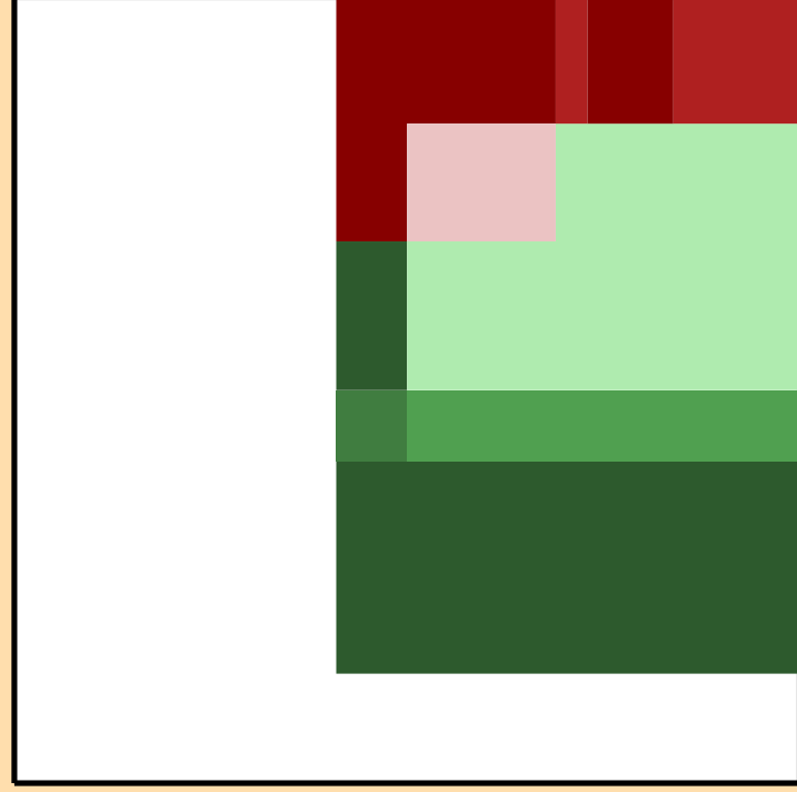
\Delta\sigma/\sigma vs. E for ^{226}\text{Po}(n,p)
