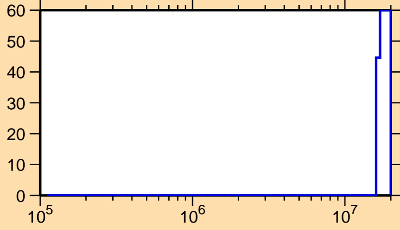
\Delta\sigma/\sigma vs. E for ^{226}\text{Po}(n,\text{f})
