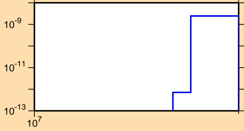
\sigma vs. E for ^{226}\text{Po}(n,\text{nd})
