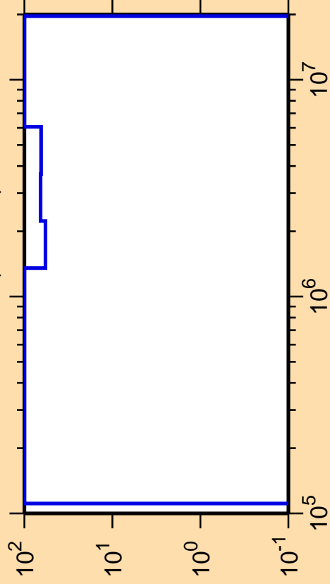
\Delta\sigma/\sigma vs. E for ^{226}\text{Po}(n,\text{inel.})
