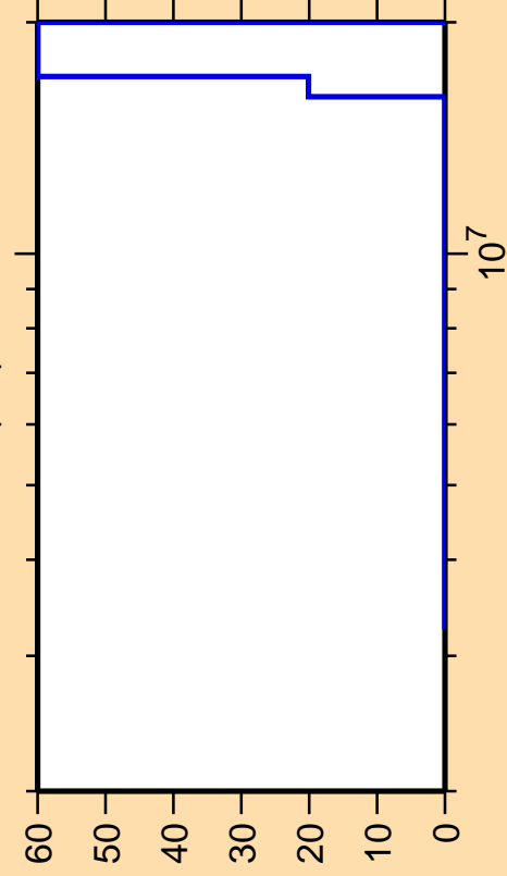
\Delta\sigma/\sigma vs. E for ^{227}\text{Po}(n,f)
