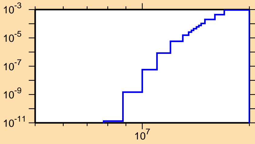
\sigma vs. E for ^{227}\text{Po}(n,p)
