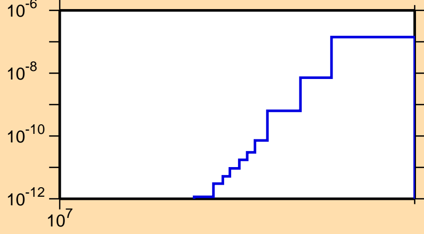
\sigma vs. E for ^{227}\text{Po}(n,2n\alpha)
