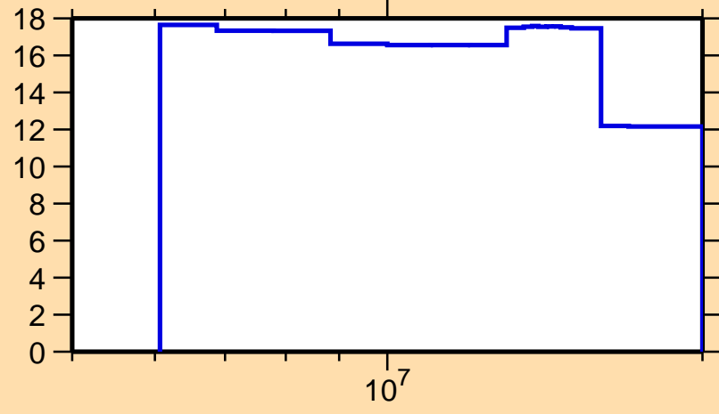
\Delta\sigma/\sigma vs. E for ^{227}\text{Po}(n,\text{nonel.})
