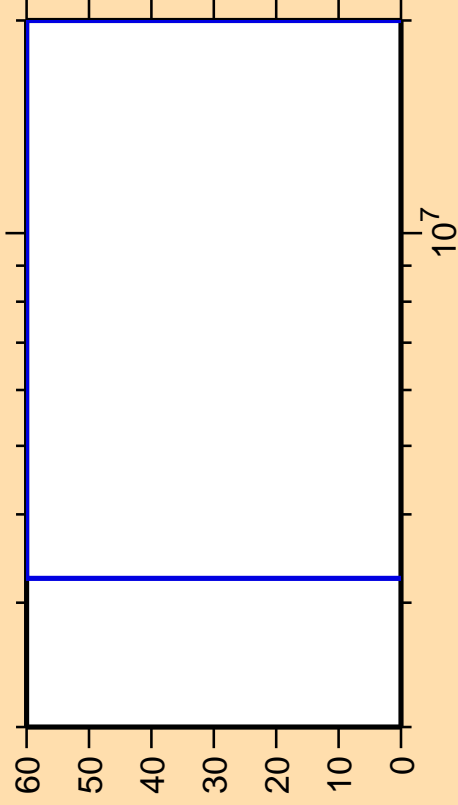
\Delta\sigma/\sigma vs. E for ^{227}\text{Po}(n,n\text{cont.})
