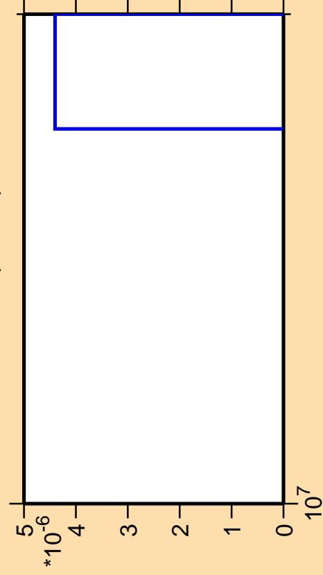
\Delta\sigma/\sigma vs. E for ^{227}\text{Po} (mt 42)
