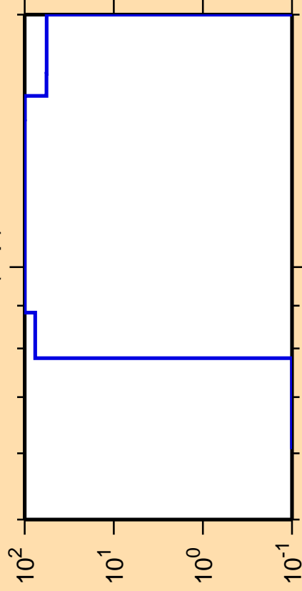
\Delta\sigma/\sigma vs. E for ^{227}\text{Po}(n,p)
