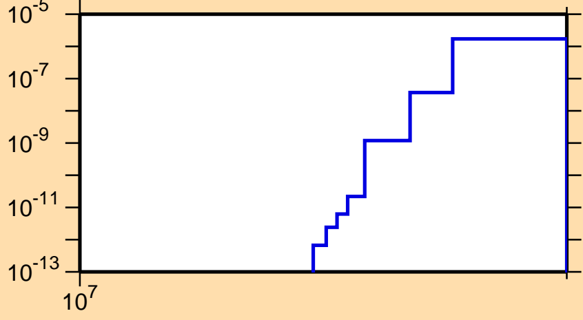
\sigma vs. E for ^{227}\text{Po}(n,nt)
