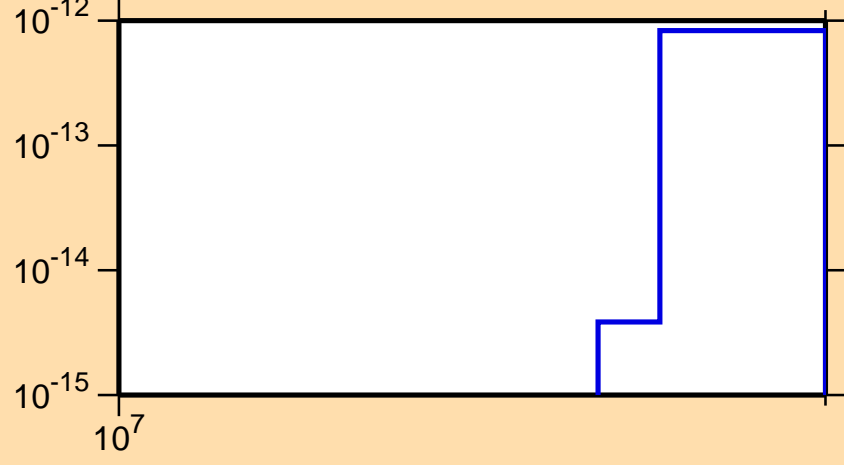
\sigma vs. E for ^{227}\text{Po}(n,3n\alpha)
