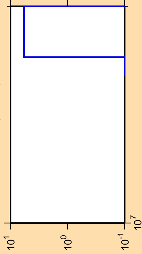
\Delta\sigma/\sigma vs. E for ^{227}\text{Po}(n,3n\alpha)
