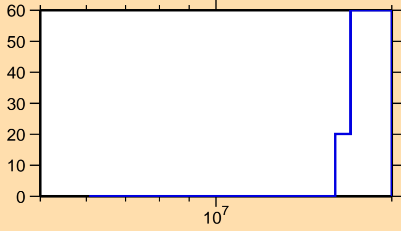
\Delta\sigma/\sigma vs. E for ^{227}\text{Po}(n,f)
