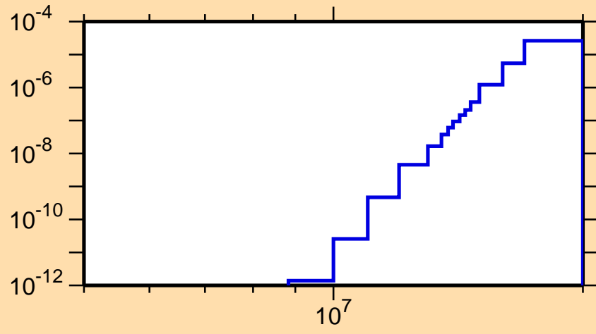
\sigma vs. E for ^{227}\text{Po}(n,n\alpha)
