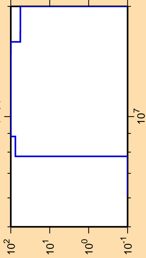
\Delta\sigma/\sigma vs. E for ^{227}\text{Po}(n,p)
