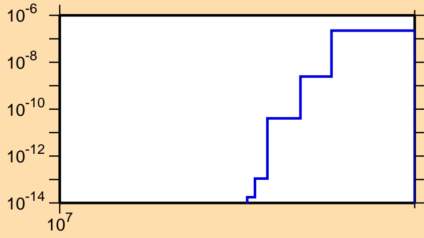
\sigma vs. E for ^{227}\text{Po}(n,\text{nd})
