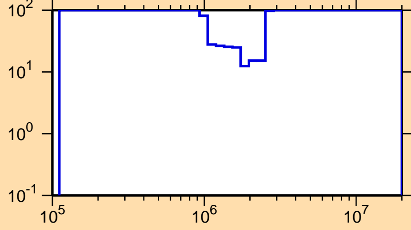
\Delta\sigma/\sigma vs. E for ^{227}\text{Po}(n,\text{inel.})
