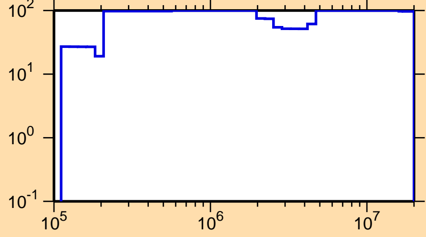
\Delta\sigma/\sigma vs. E for ^{227}\text{Po}(n,\text{el.})
