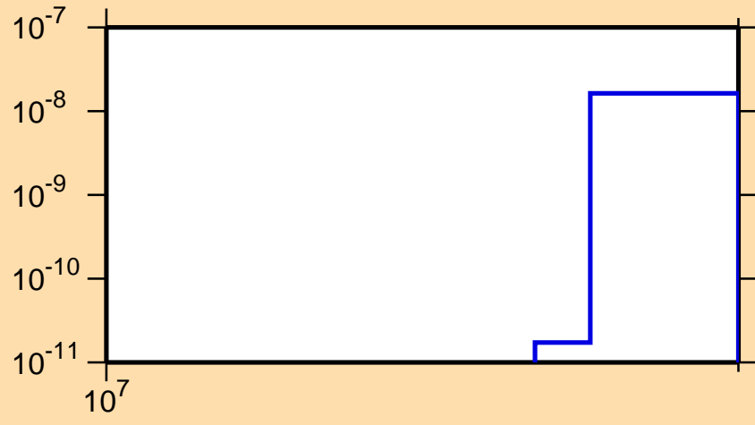
\sigma vs. E for ^{227}\text{Po}(n,2np)
