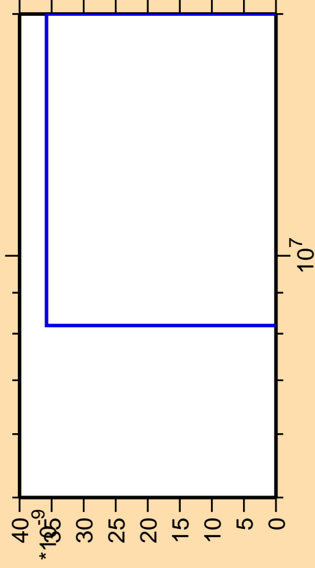
\Delta\sigma/\sigma vs. E for ^{227}\text{Po} (mt 42)
