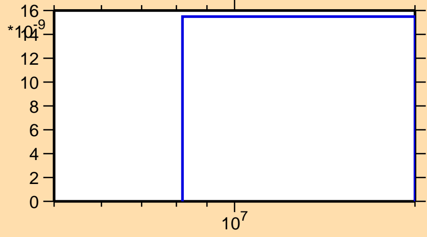
\sigma vs. E for ^{227}\text{Po}(n,\text{nt})
