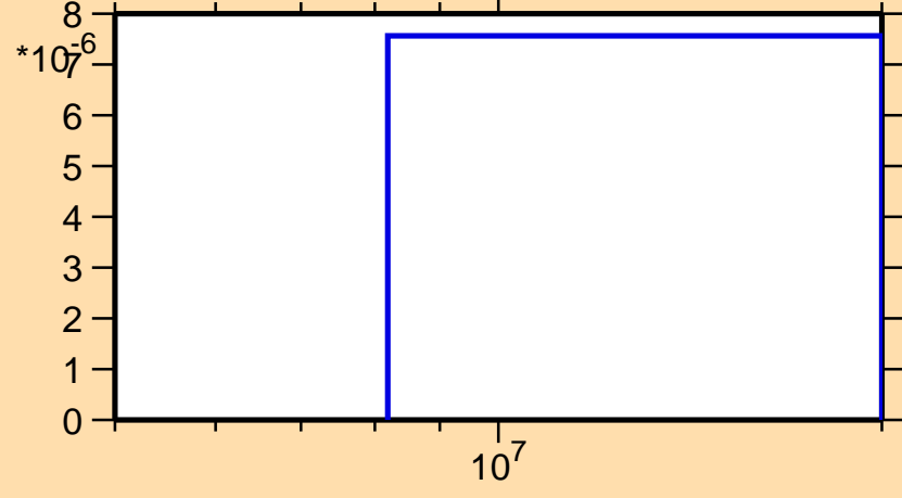
\sigma vs. E for ^{227}\text{Po}(n,t)
