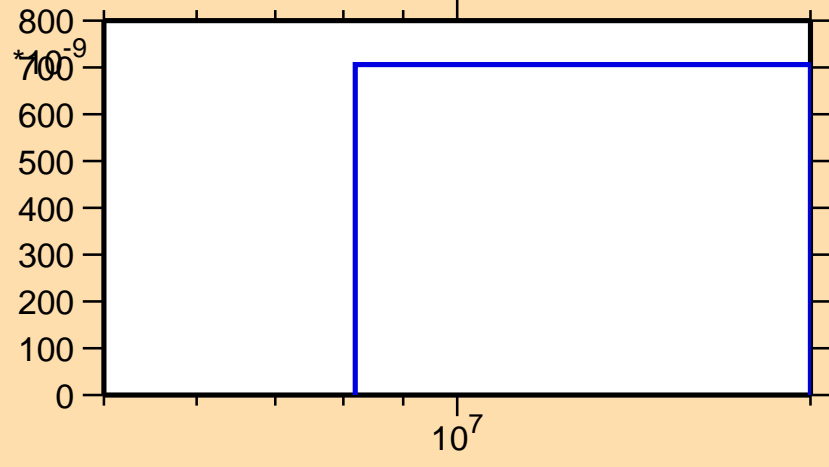
\sigma vs. E for ^{227}\text{Po}(n,np)
