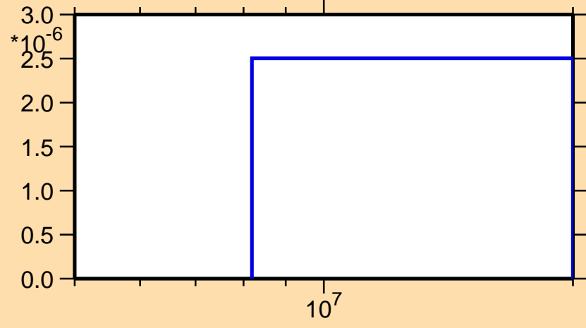
\sigma vs. E for ^{227}\text{Po}(n,d)
