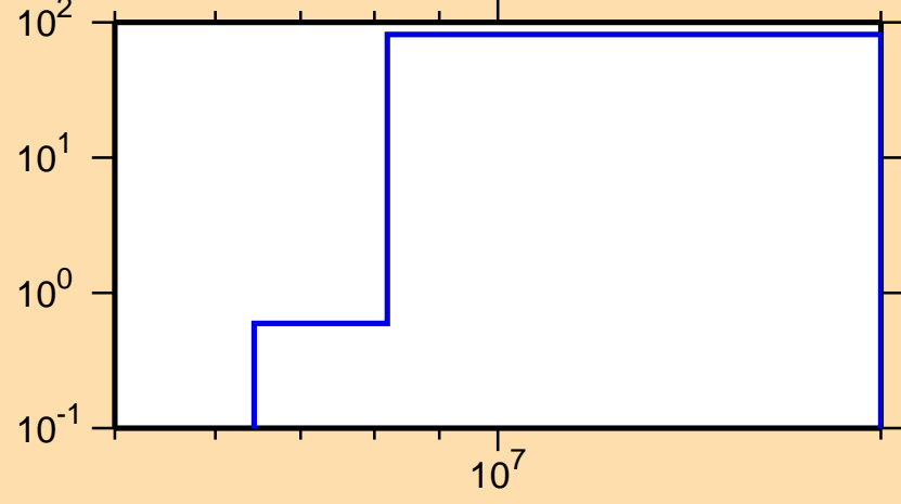
\Delta\sigma/\sigma vs. E for ^{227}\text{Po}(n,p)
