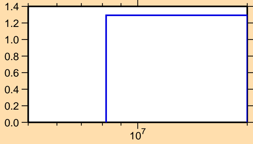
\sigma vs. E for ^{227}\text{Po}(n,3n)
