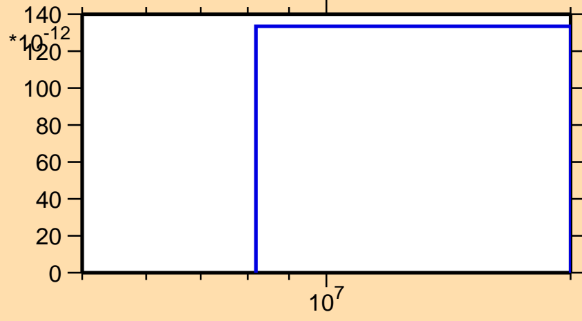
\sigma vs. E for ^{227}\text{Po}(n,2np)
