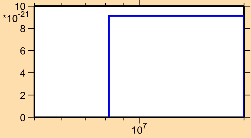
\sigma vs. E for ^{227}\text{Po} (mt 42)
