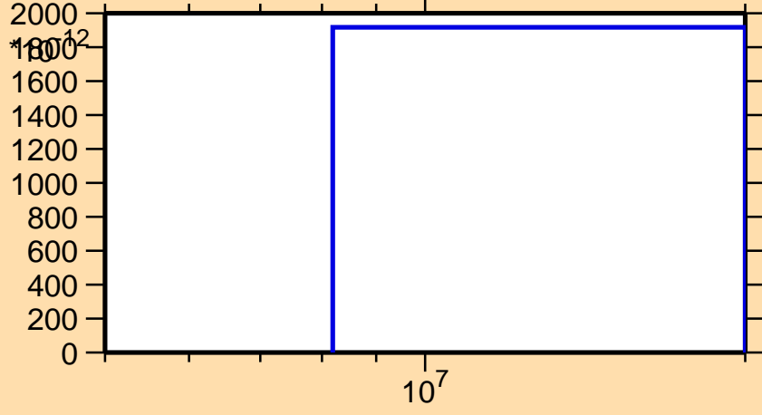
\sigma vs. E for ^{227}\text{Po}(n,\text{nd})
