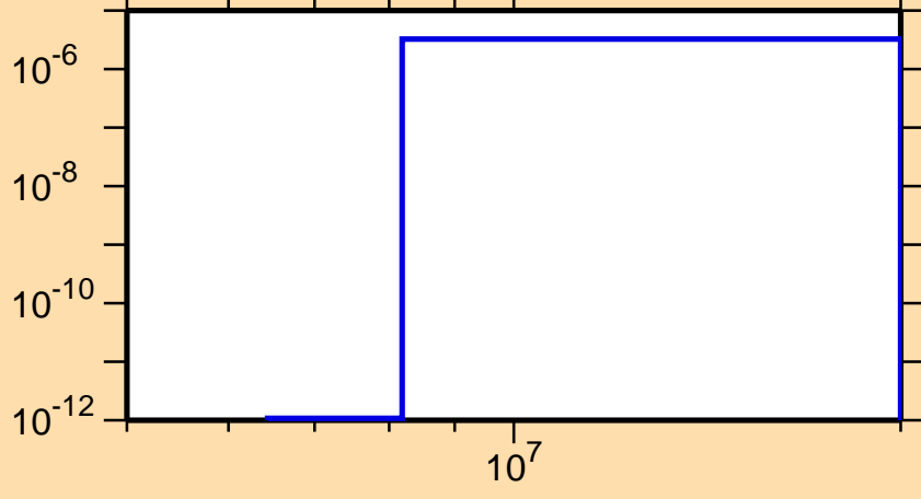
\sigma vs. E for ^{227}\text{Po}(n,\alpha)
