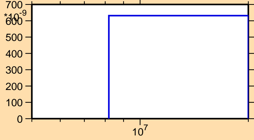
\sigma vs. E for ^{227}\text{Po}(n,n\alpha)
