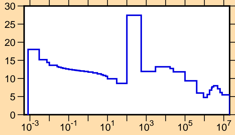
\sigma vs. E for ^{227}\text{Po}(n,\text{tot.})
