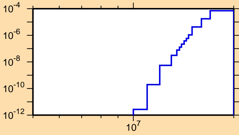
\sigma vs. E for ^{175}\text{Pt}(n,\text{pt})
