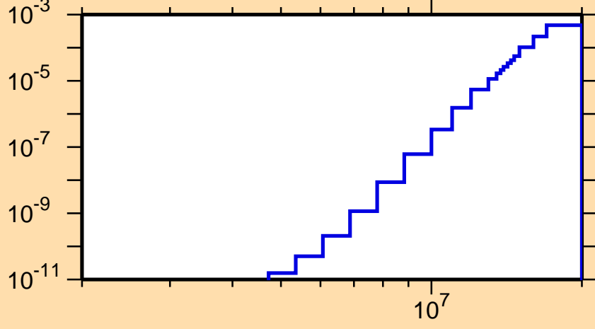
\sigma vs. E for ^{175}\text{Pt}(n,\text{He}3)
