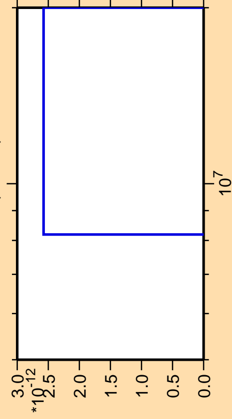
\Delta\sigma/\sigma vs. E for ^{175}\text{Pt}(\text{mt } 11)
