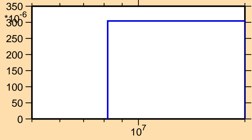
\sigma vs. E for ^{175}\text{Pt}(n,2np)
