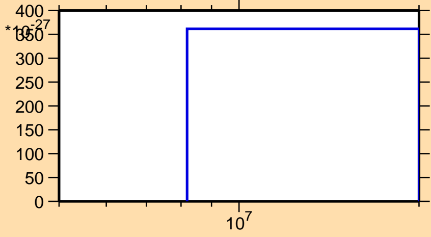
\sigma vs. E for ^{175}\text{Pt}(\text{mt } 11)
