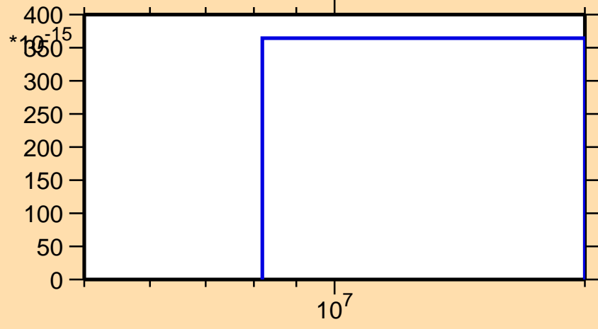
\sigma vs. E for ^{175}\text{Pt}(n,nt)
