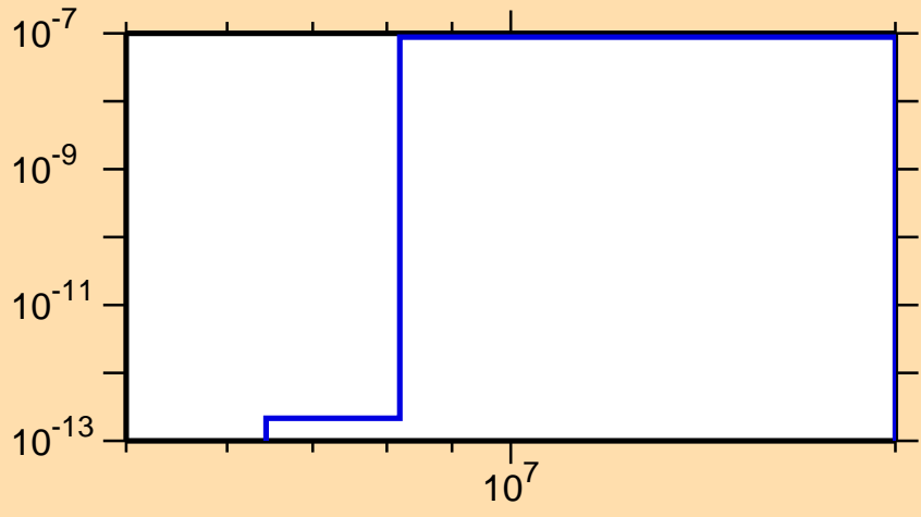
\sigma vs. E for ^{175}\text{Pt}(\text{mt117})
