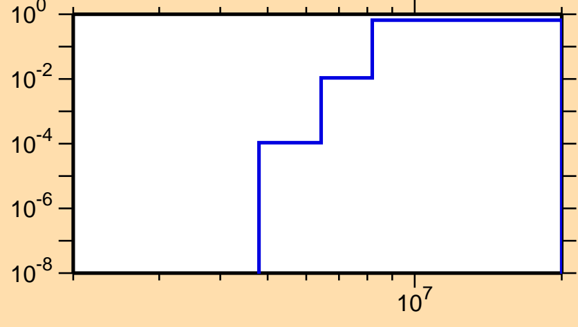
\sigma vs. E for ^{175}\text{Pt}(n,np)
