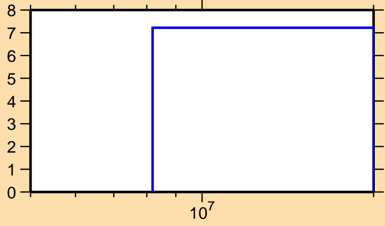
\Delta\sigma/\sigma vs. E for ^{175}\text{Pt}(n,\text{tot.})
