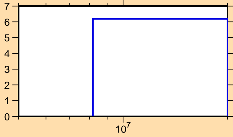
\Delta\sigma/\sigma vs. E for ^{175}\text{Pt}(n,\text{el.})
