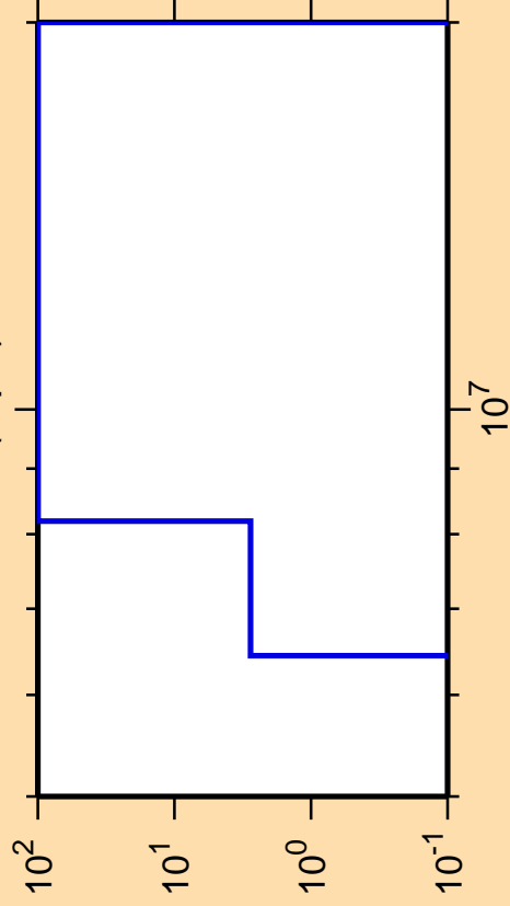
\Delta\sigma/\sigma vs. E for ^{175}\text{Pt}(n,\text{pd})
