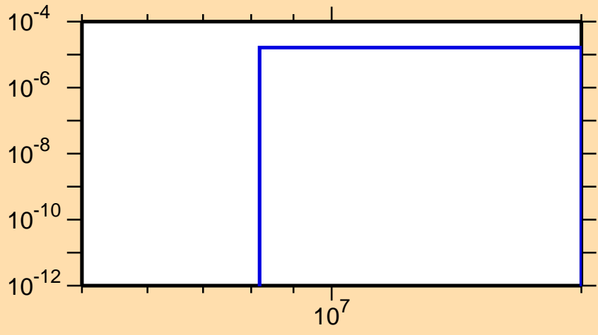
\sigma vs. E for ^{175}\text{Pt}(n,\text{pd})
