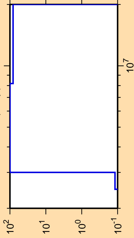
\Delta\sigma/\sigma vs. E for ^{175}\text{Pt}(n,np)
