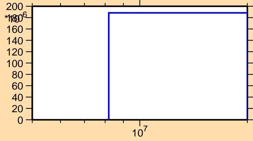
\sigma vs. E for ^{175}\text{Pt}(n,2n\alpha)
