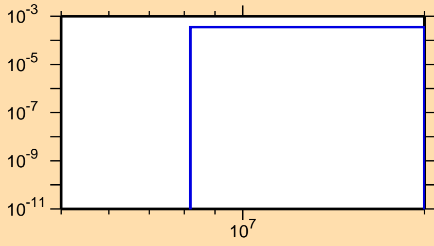
\sigma vs. E for ^{175}\text{Pt}(n,t)
