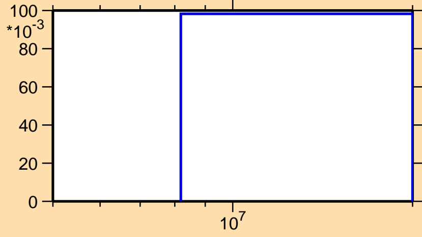
\sigma vs. E for ^{175}\text{Pt}(n,2n)
