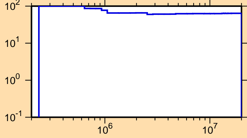
\Delta\sigma/\sigma vs. E for ^{176}\text{Pt}(n,n_1)
