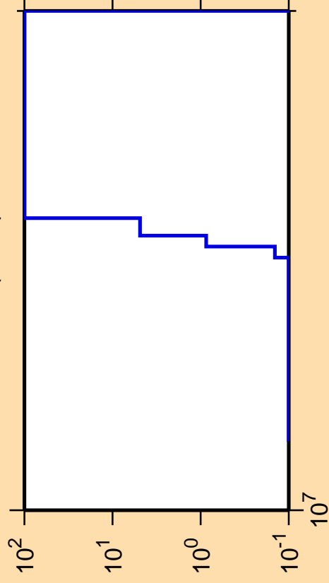
\Delta\sigma/\sigma vs. E for ^{176}\text{Pt}(n,nd)
