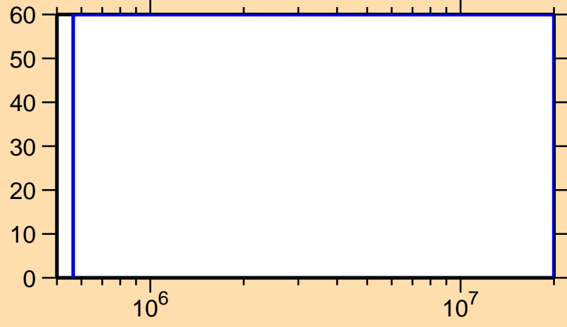
\Delta\sigma/\sigma vs. E for ^{176}\text{Pt}(n,ncont.)
