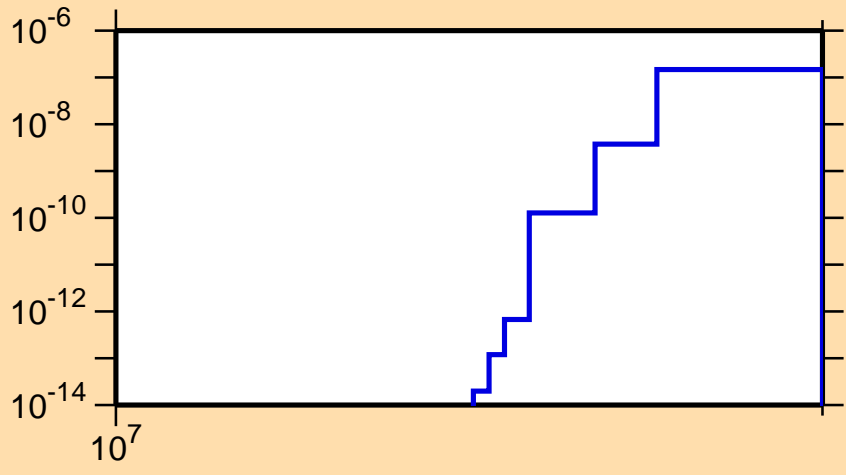
\sigma vs. E for ^{176}\text{Pt}(n,nd)
