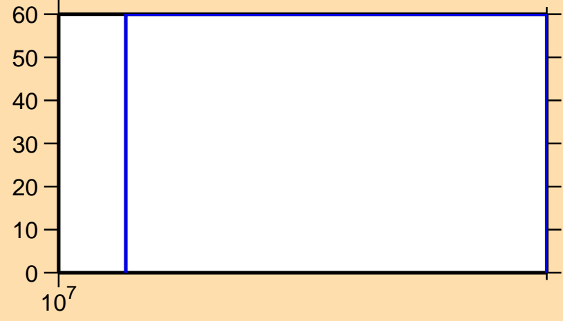
\Delta\sigma/\sigma vs. E for ^{176}\text{Pt}(n,\text{inel.})
