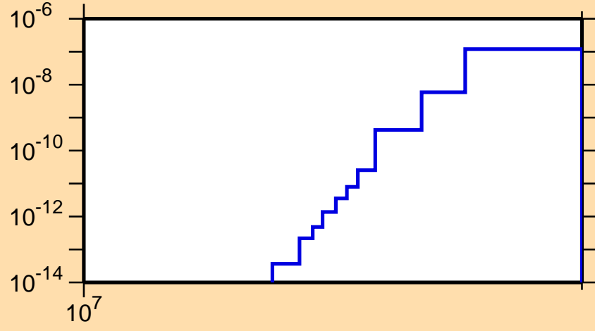
\sigma vs. E for ^{176}\text{Pt}(n,pt)
