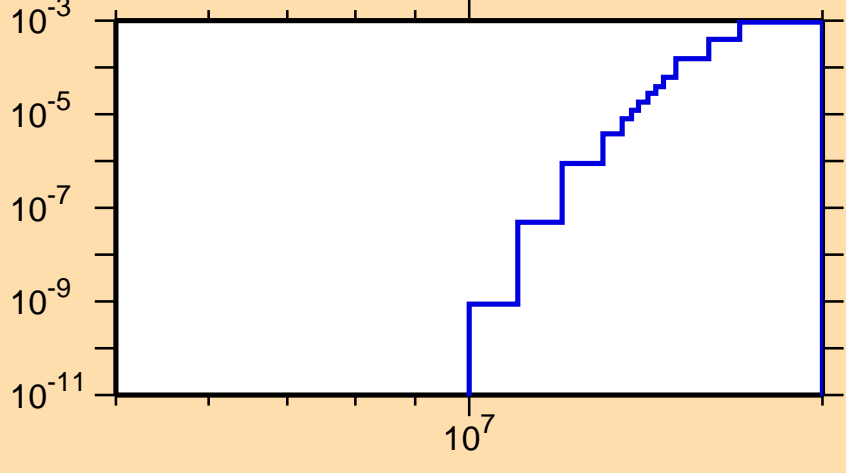
\sigma vs. E for ^{176}\text{Pt}(n,t)
