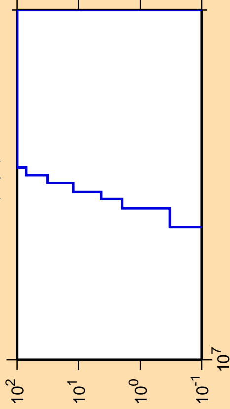
\Delta\sigma/\sigma vs. E for ^{176}\text{Pt}(n,pt)
