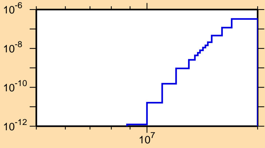
\sigma vs. E for ^{176}\text{Pt}(\text{mt117})
