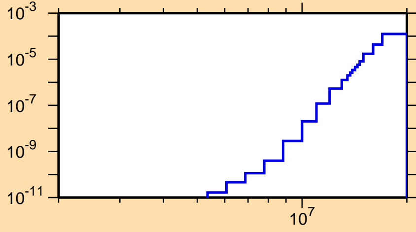
\sigma vs. E for ^{176}\text{Pt}(n,\text{He}3)
