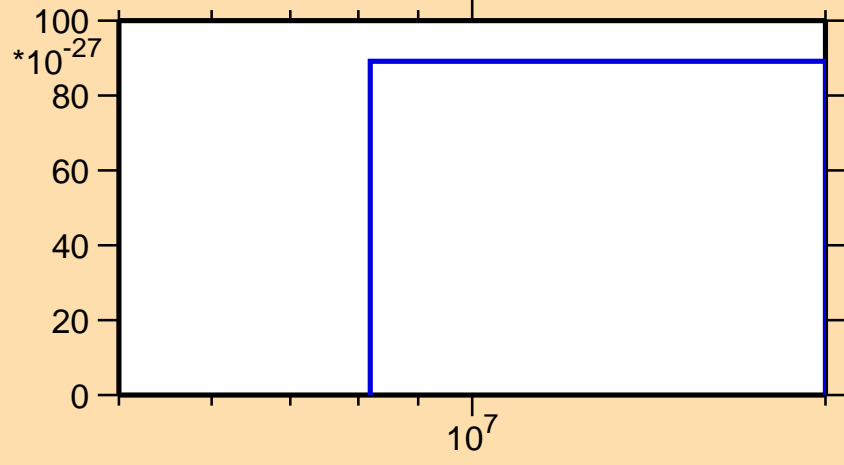
\sigma vs. E for ^{176}\text{Pt}(\text{mt } 11)
