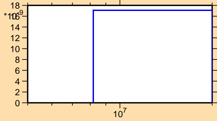
\sigma vs. E for ^{176}\text{Pt}(\text{mt117})
