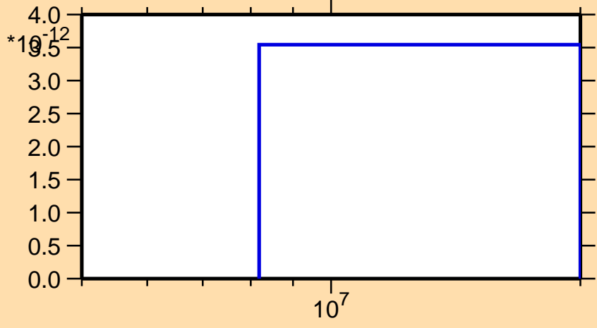
\sigma vs. E for ^{176}\text{Pt}(\text{mt } 34)
