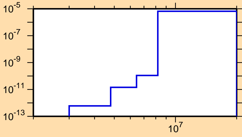
\sigma vs. E for ^{176}\text{Pt}(n,\text{He}3)
