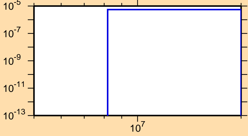
\sigma vs. E for ^{176}\text{Pt}(n,\text{pd})
