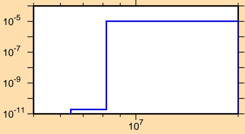
\sigma vs. E for ^{176}\text{Pt}(\text{mt } 45)
