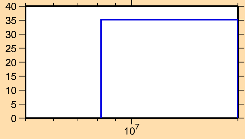
\Delta\sigma/\sigma vs. E for ^{176}\text{Pt}(n,\text{tot.})
