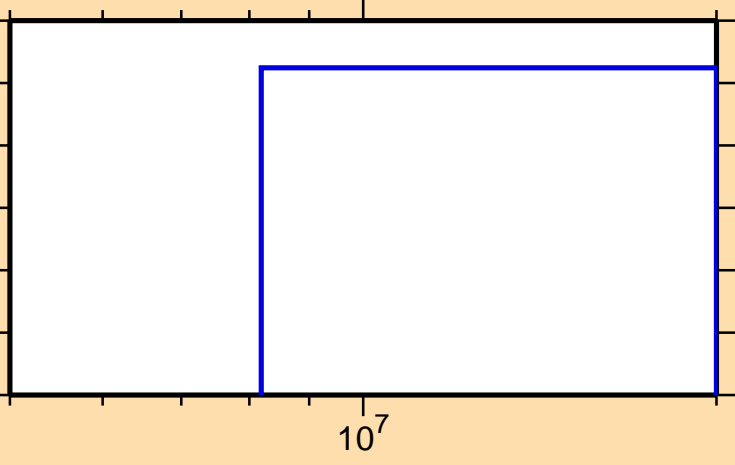
\sigma vs. E for ^{176}\text{Pt}(n,t)
