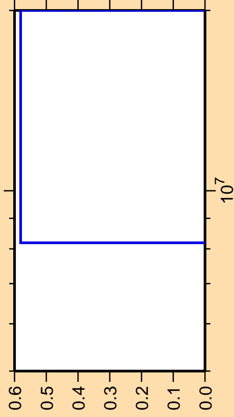
\Delta\sigma/\sigma vs. E for ^{176}\text{Pt}(n,nt)
