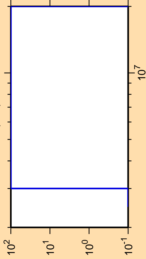
\Delta\sigma/\sigma vs. E for ^{176}\text{Pt}(n,d)
