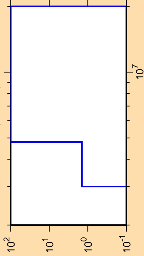
\Delta\sigma/\sigma vs. E for ^{176}\text{Pt}(n,\text{He}3)
