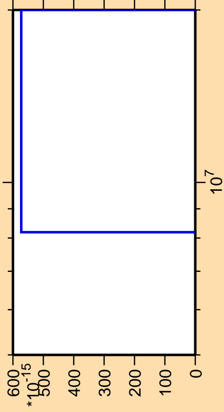
\Delta\sigma/\sigma vs. E for ^{176}\text{Pt}(\text{mt } 11)
