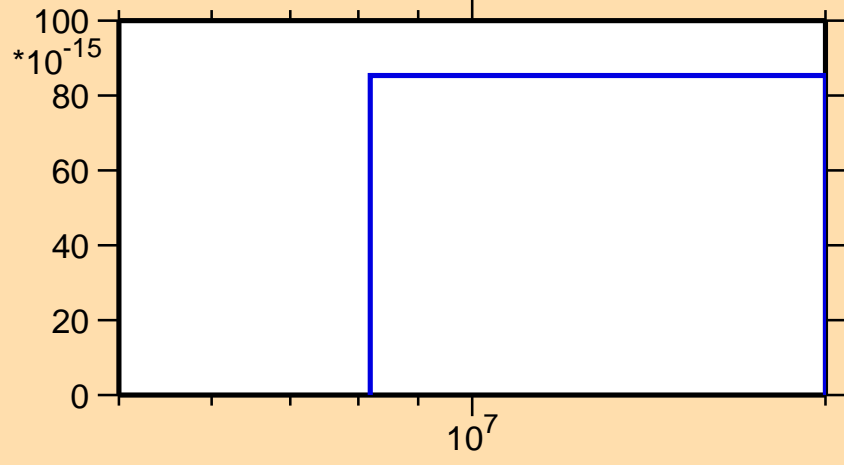
\sigma vs. E for ^{176}\text{Pt}(n,nt)
