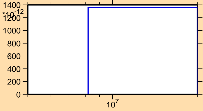
\sigma vs. E for ^{176}\text{Pt}(n,\text{nd})
