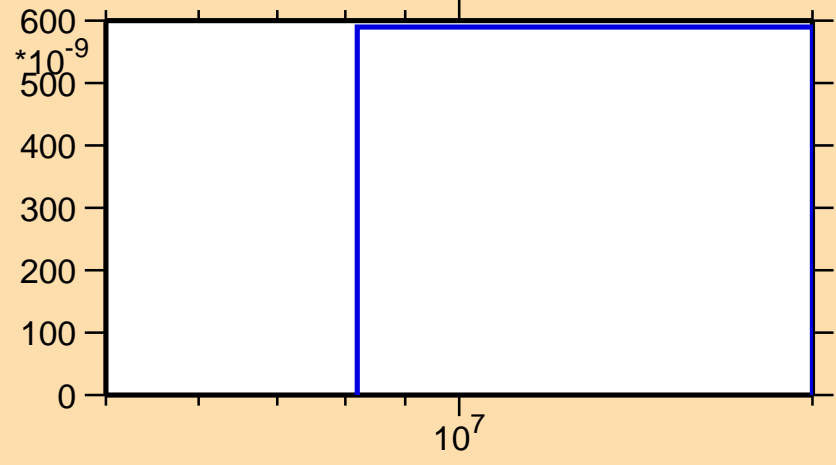
\sigma vs. E for ^{176}\text{Pt}(n,2np)
