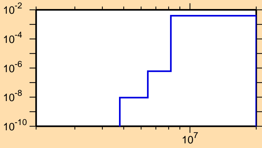
\sigma vs. E for ^{176}\text{Pt}(n,d)
