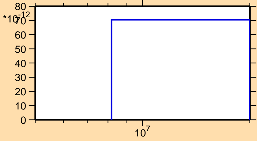
\sigma vs. E for ^{176}\text{Pt}(n,3n)
