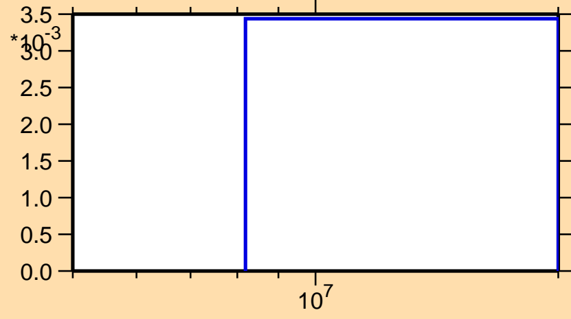
\sigma vs. E for ^{176}\text{Pt}(n,2n\alpha)
