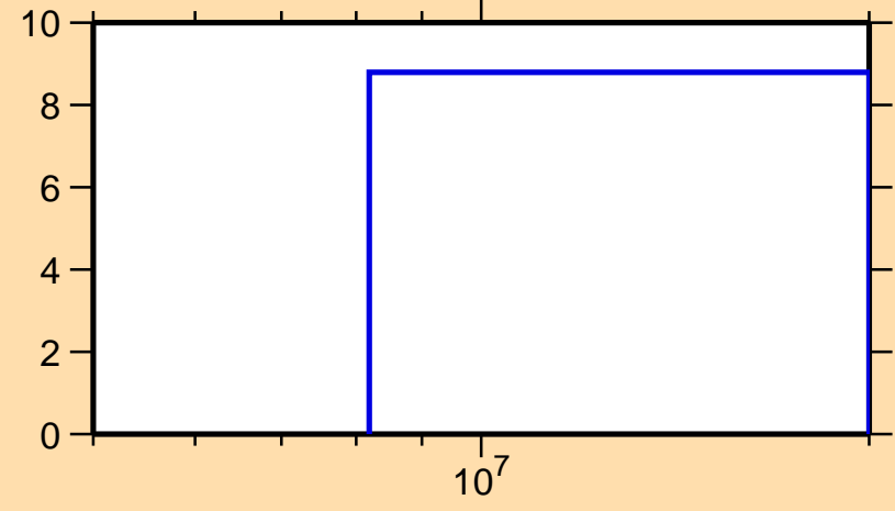
\Delta\sigma/\sigma vs. E for ^{176}\text{Pt}(n,\text{nonel.})
