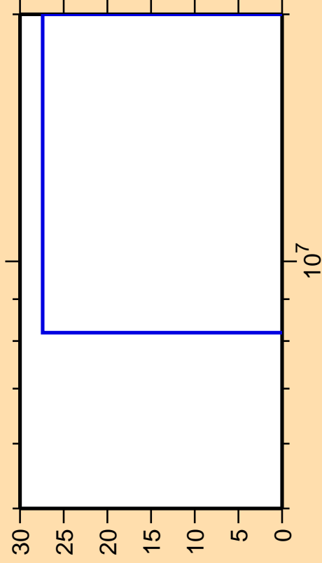
\Delta\sigma/\sigma vs. E for ^{176}\text{Pt}(\text{mt } 34)
