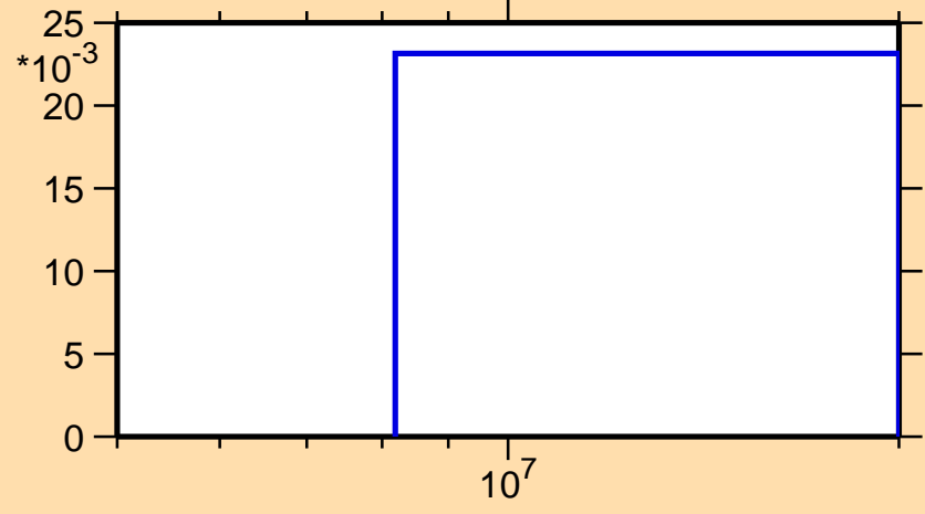
\sigma vs. E for ^{176}\text{Pt}(n,2n)
