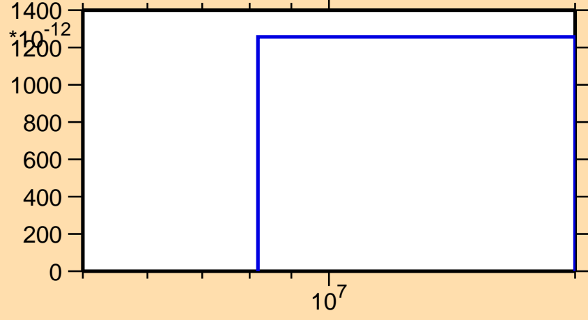
\sigma vs. E for ^{176}\text{Pt}(n,\text{pt})
