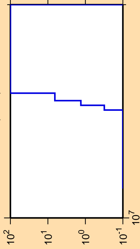
\Delta\sigma/\sigma vs. E for ^{178}\text{Pt}(n,nd)
