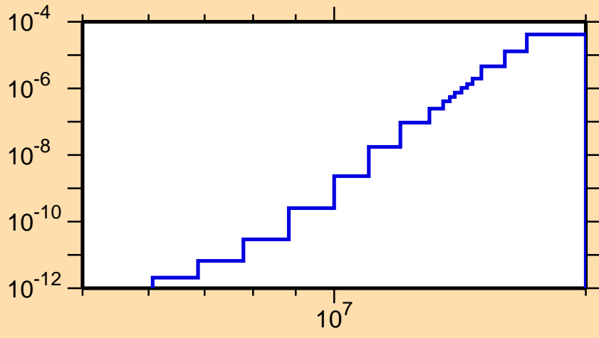
\sigma vs. E for ^{178}\text{Pt}(n,\text{He}3)
