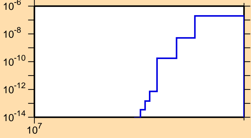
\sigma vs. E for ^{178}\text{Pt}(n,nd)
