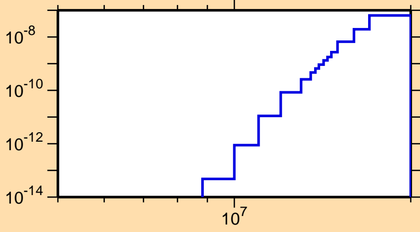
\sigma vs. E for ^{178}\text{Pt}(\text{mt117})
