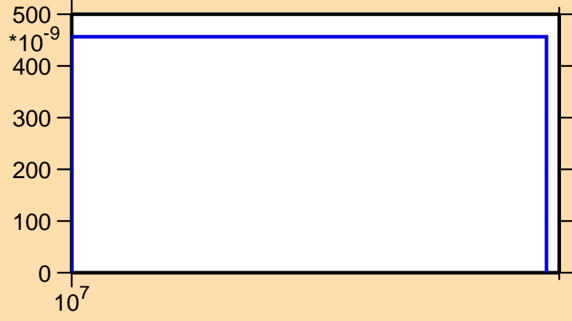
\sigma vs. E for ^{178}\text{Pt}(n,2np)
