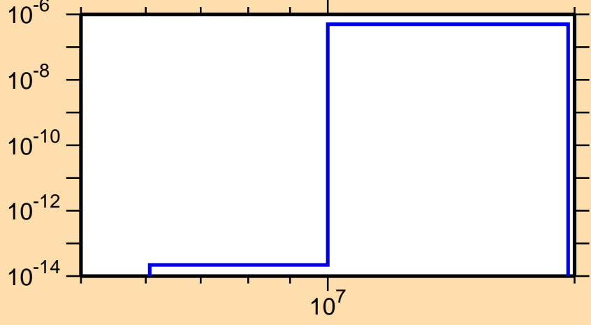
\sigma vs. E for ^{178}\text{Pt}(n,pd)
