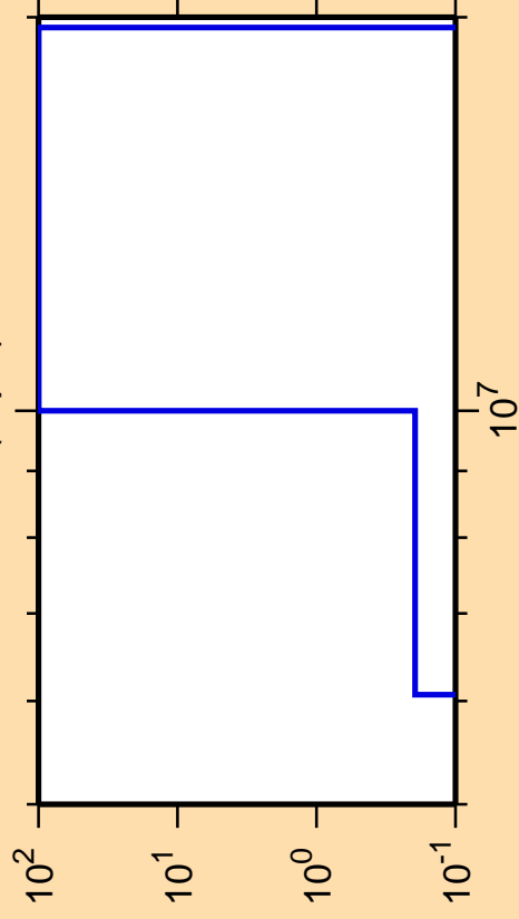
\Delta\sigma/\sigma vs. E for ^{178}\text{Pt}(n,pd)
