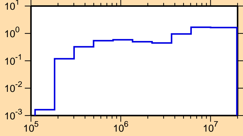
\sigma vs. E for ^{178}\text{Pt}(n,\text{inel.})
