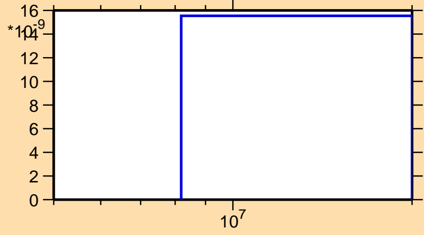
\sigma vs. E for ^{178}\text{Pt}(n,3n)
