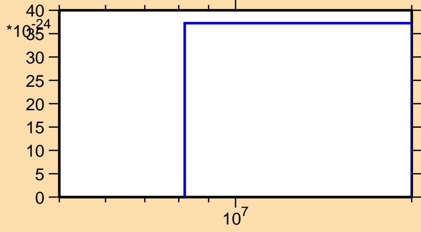
\sigma vs. E for ^{178}\text{Pt}(\text{mt } 11)
