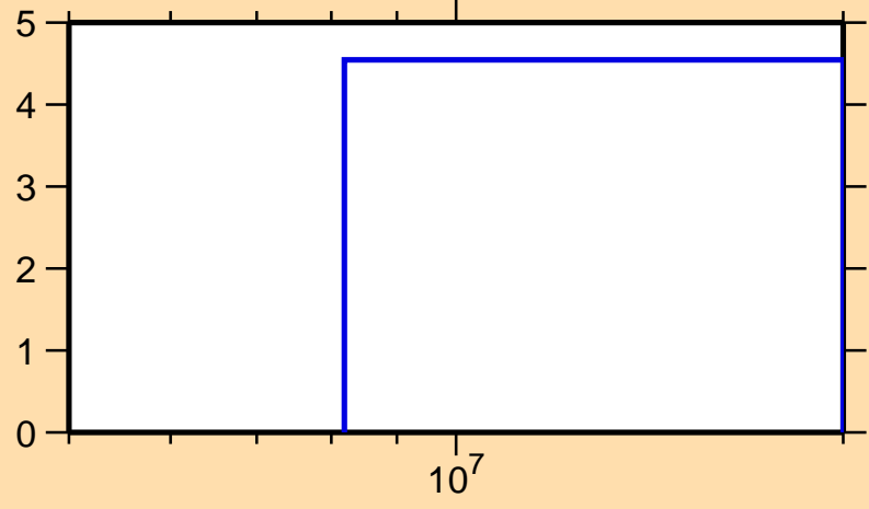
\Delta\sigma/\sigma vs. E for ^{178}\text{Pt}(n,\text{nonel.})
