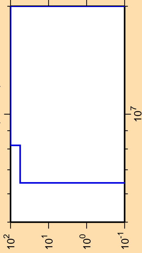
\Delta\sigma/\sigma vs. E for ^{178}\text{Pt}(n,\text{He}3)
