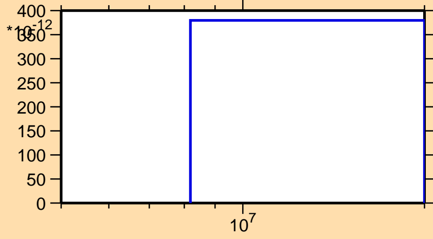
\sigma vs. E for ^{178}\text{Pt}(n,\text{pt})
