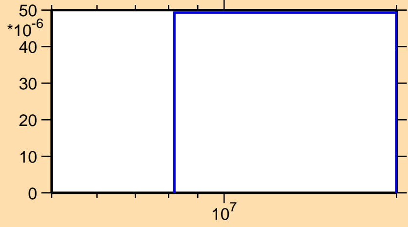
\sigma vs. E for ^{178}\text{Pt}(n,t)
