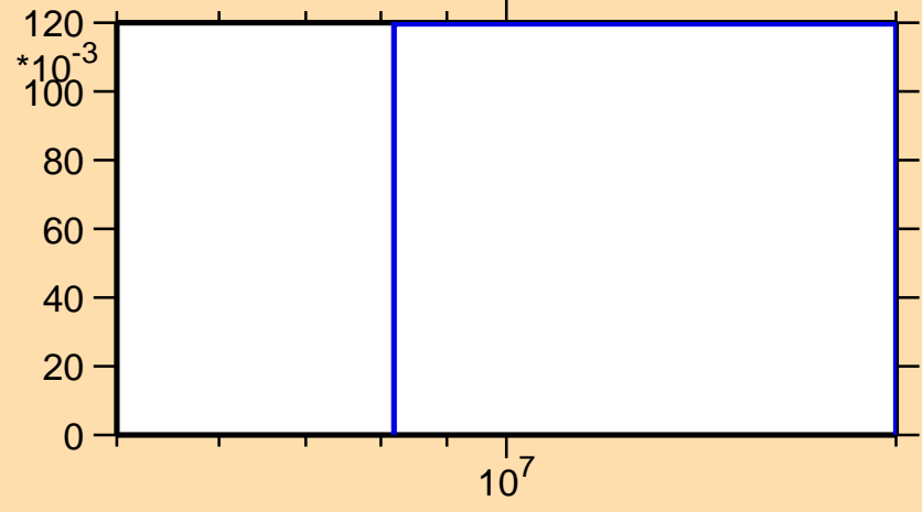
\sigma vs. E for ^{178}\text{Pt}(n,2n)
