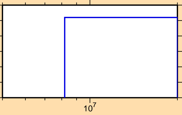
\sigma vs. E for ^{178}\text{Pt}(\text{mt117})
