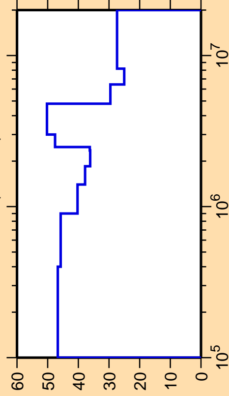
\Delta\sigma/\sigma vs. E for ^{178}\text{Pt}(n,\text{inel.})
