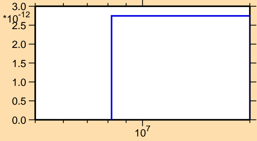
\sigma vs. E for ^{178}\text{Pt}(\text{mt } 34)
