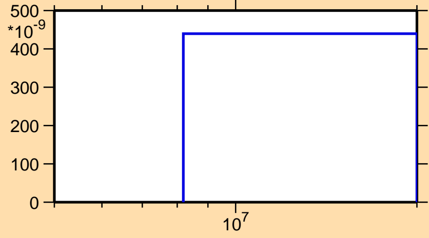
\sigma vs. E for ^{178}\text{Pt}(n,2np)
