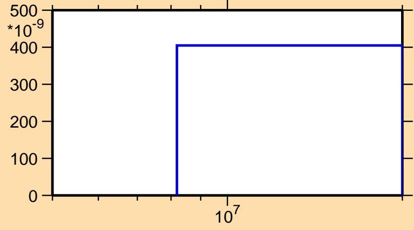
\sigma vs. E for ^{178}\text{Pt}(n,\text{pd})
