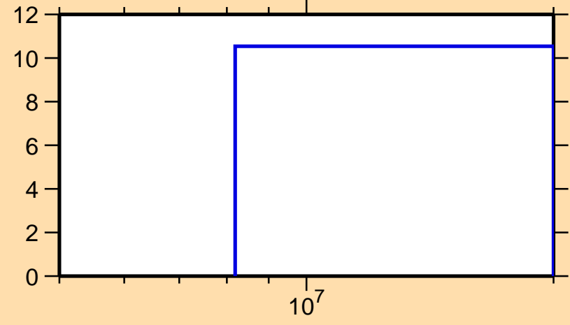
\Delta\sigma/\sigma vs. E for ^{178}\text{Pt}(n,\text{el.})
