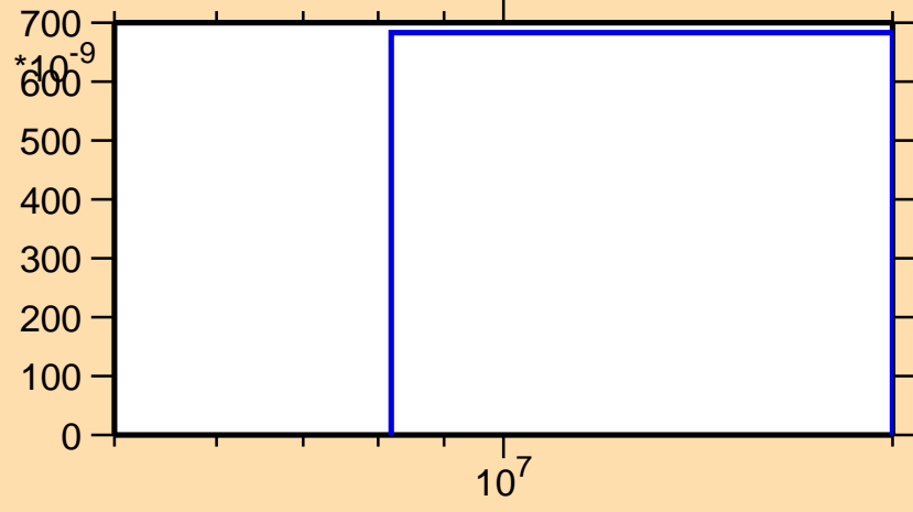
\sigma vs. E for ^{178}\text{Pt}(n,2n\alpha)
