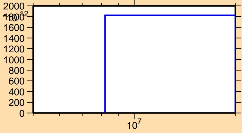
\sigma vs. E for ^{178}\text{Pt}(n,\text{nd})
