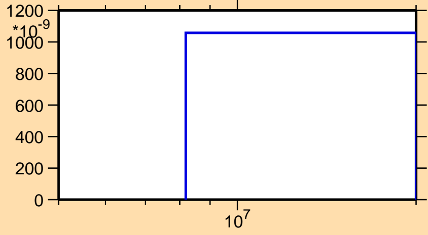
\sigma vs. E for ^{178}\text{Pt}(\text{mt } 45)
