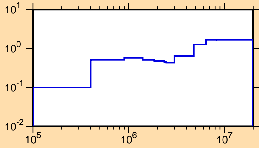
\sigma vs. E for ^{178}\text{Pt}(n,\text{inel.})
