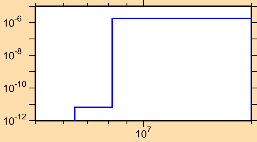
\sigma vs. E for ^{178}\text{Pt}(n,\text{He}3)
