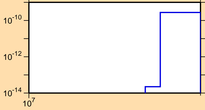
\sigma vs. E for ^{181}\text{Pt}(n,nt)
