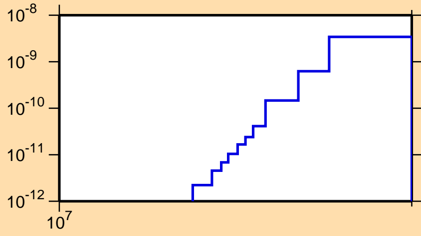
\sigma vs. E for ^{181}\text{Pt}(\text{mt117})
