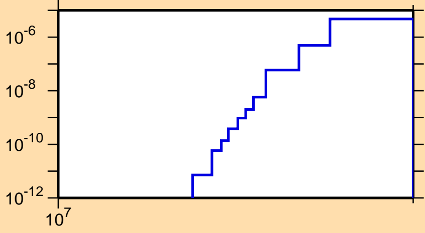
\sigma vs. E for ^{181}\text{Pt}(n,nd)
