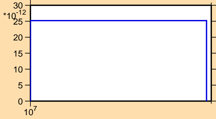
\sigma vs. E for ^{181}\text{Pt} (mt 34)
