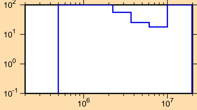
\Delta\sigma/\sigma vs. E for ^{181}\text{Pt}(n,n\text{cont.})
