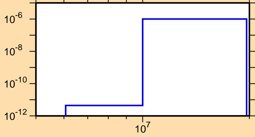
\sigma vs. E for ^{181}\text{Pt}(n,\text{He}3)
