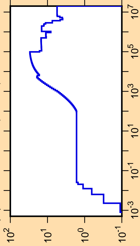
\Delta\mu/\mu vs. E for ^{182}\text{Pt}(\text{mt251})
