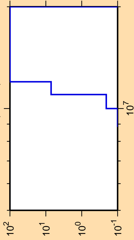
\Delta\sigma/\sigma vs. E for ^{182}\text{Pt}(\text{mt } 45)
