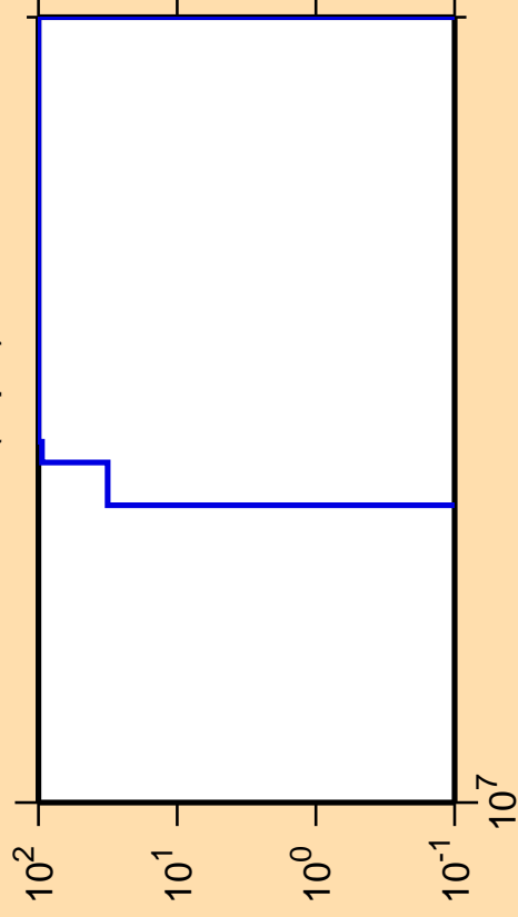
\Delta\sigma/\sigma vs. E for ^{182}\text{Pt}(n,pd)
