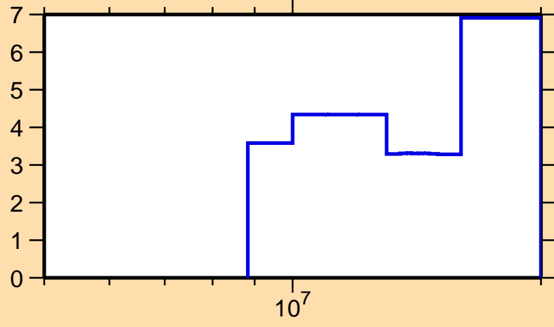
\Delta\sigma/\sigma vs. E for ^{182}\text{Pt}(n,\text{el.})
