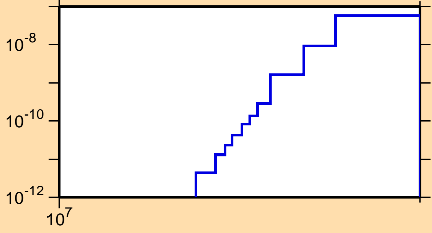
\sigma vs. E for ^{182}\text{Pt}(n,pd)
