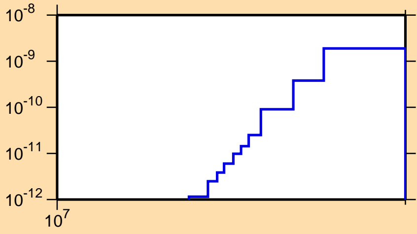
\sigma vs. E for ^{182}\text{Pt}(\text{mt117})
