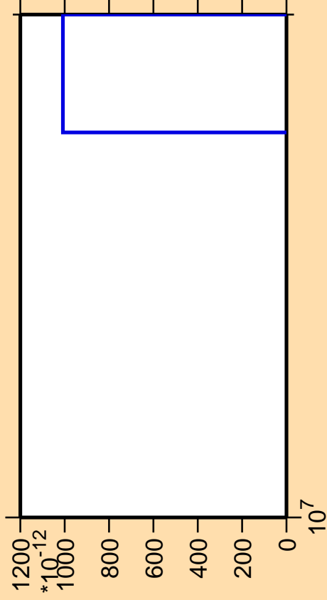
\Delta\sigma/\sigma vs. E for ^{182}\text{Pt}(\text{mt } 11)
