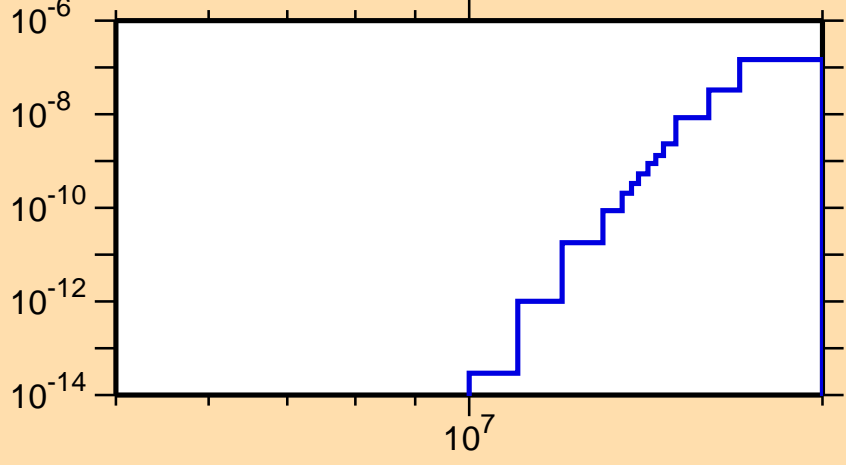
\sigma vs. E for ^{182}\text{Pt}(\text{mt } 45)
