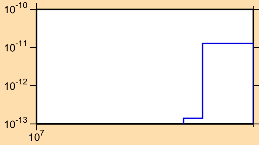
\sigma vs. E for ^{182}\text{Pt} (mt 34)
