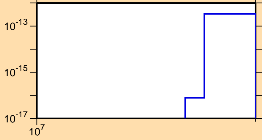
\sigma vs. E for ^{182}\text{Pt}(n,3n\alpha)
