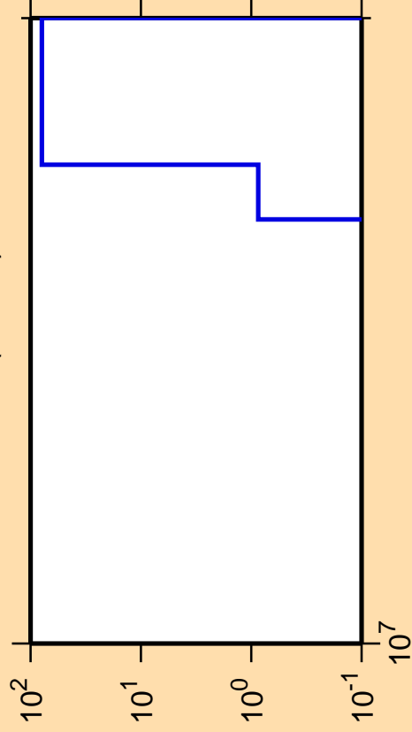
\Delta\sigma/\sigma vs. E for ^{182}\text{Pt} (mt 34)
