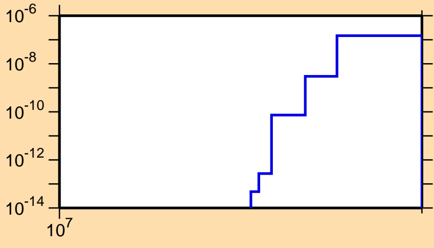
\sigma vs. E for ^{182}\text{Pt}(n,\text{nd})
