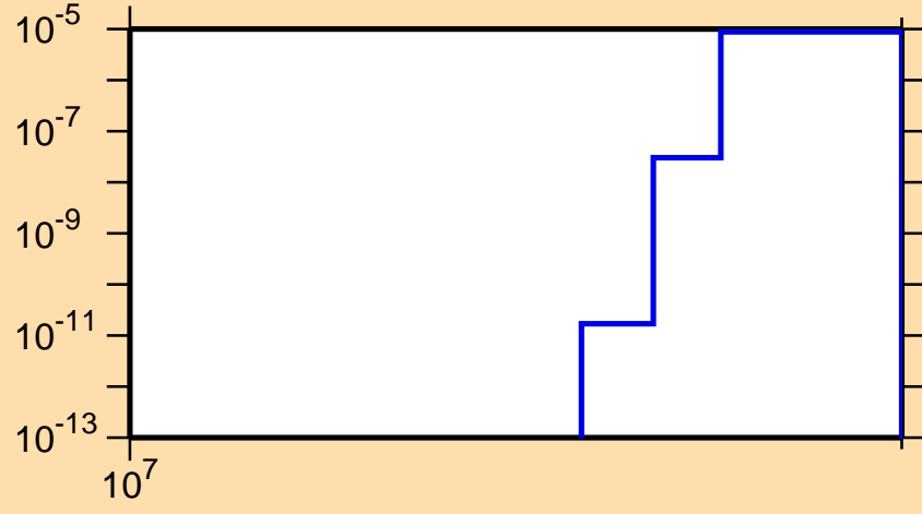
\sigma vs. E for ^{182}\text{Pt}(n,2np)
