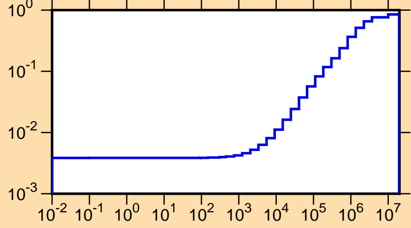
\mu vs. E for ^{182}\text{Pt}(\text{mt251})
