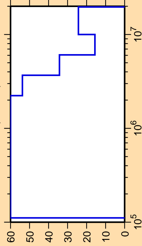
\Delta\sigma/\sigma vs. E for ^{182}\text{Pt}(n,\text{inel.})
