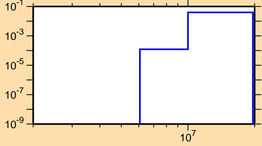
\sigma vs. E for ^{182}\text{Pt}(n,np)
