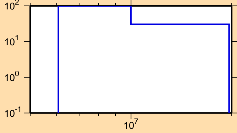
\Delta\sigma/\sigma vs. E for ^{182}\text{Pt}(n,2n)
