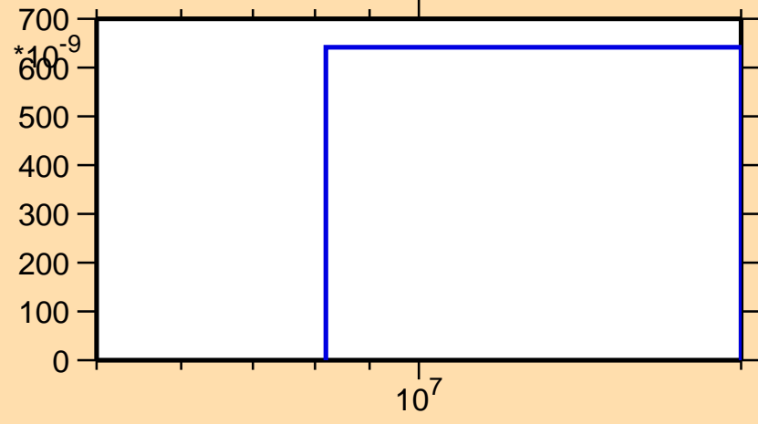
\sigma vs. E for ^{182}\text{Pt}(n,2n\alpha)
