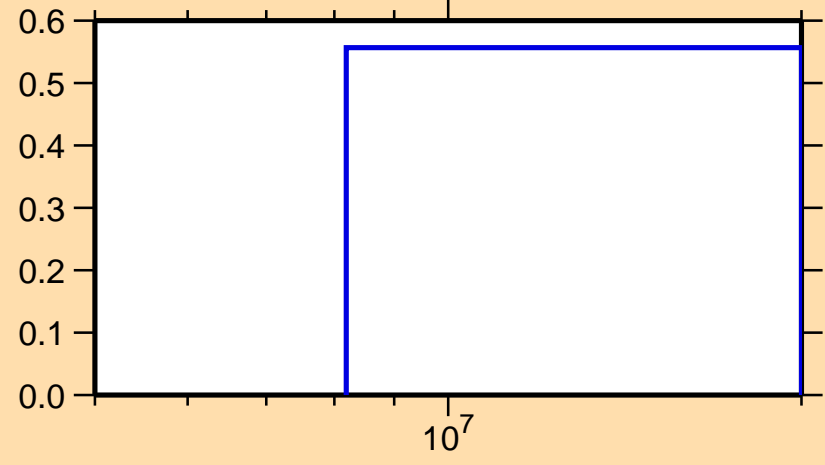
\sigma vs. E for ^{182}\text{Pt}(n,2n)
