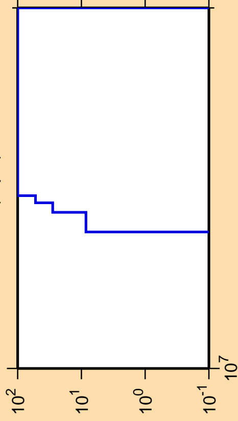
\Delta\sigma/\sigma vs. E for ^{183}\text{Pt}(n,pd)
