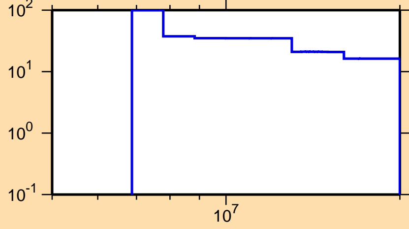
\Delta\sigma/\sigma vs. E for ^{183}\text{Pt}(n,2n)
