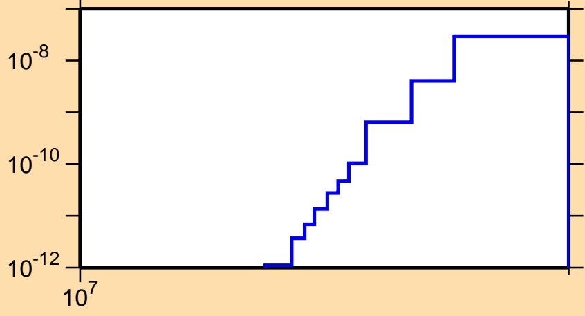
\sigma vs. E for ^{183}\text{Pt}(n,pd)
