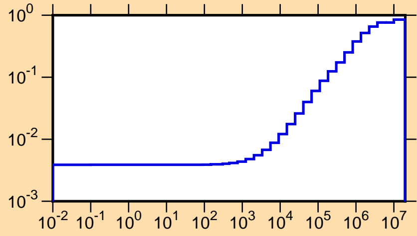
\mu vs. E for ^{183}\text{Pt}(\text{mt251})
