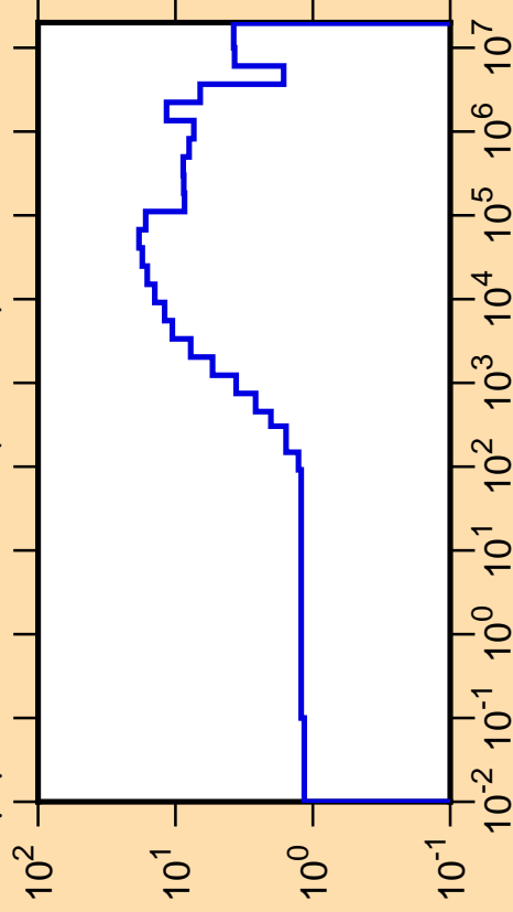
\Delta\mu/\mu vs. E for ^{183}\text{Pt}(\text{mt251})
