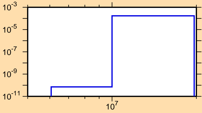
\sigma vs. E for ^{183}\text{Pt}(n,t)
