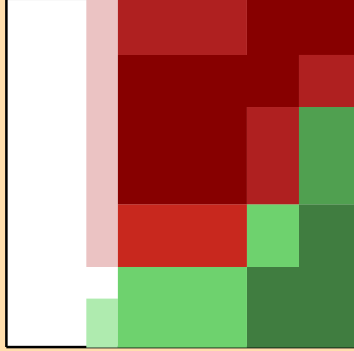
\Delta\sigma/\sigma vs. E for ^{183}\text{Pt}(n,2n)
