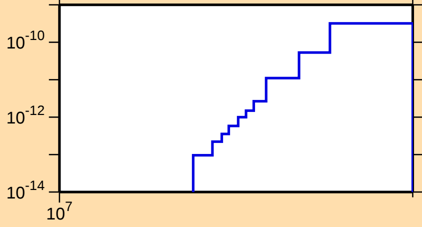
\sigma vs. E for ^{183}\text{Pt}(\text{mt117})
