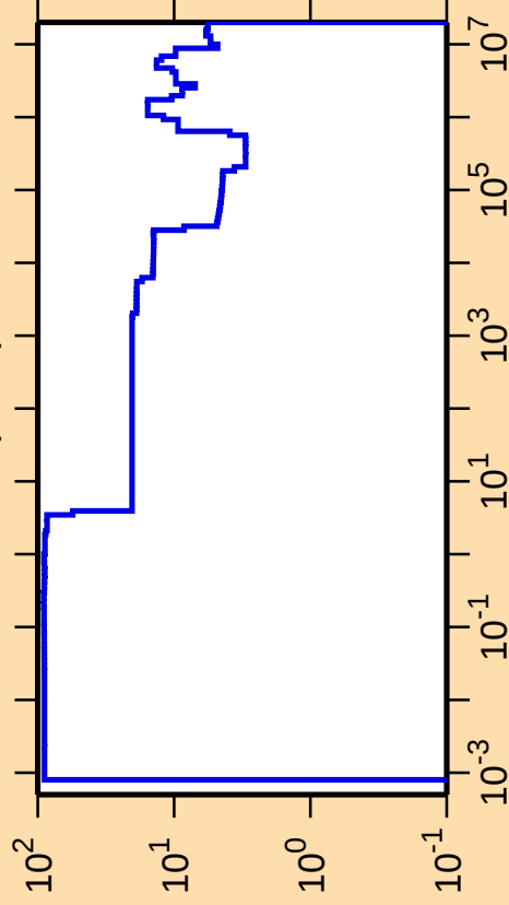
\Delta\sigma/\sigma vs. E for ^{183}\text{Pt}(n,\text{el.})
