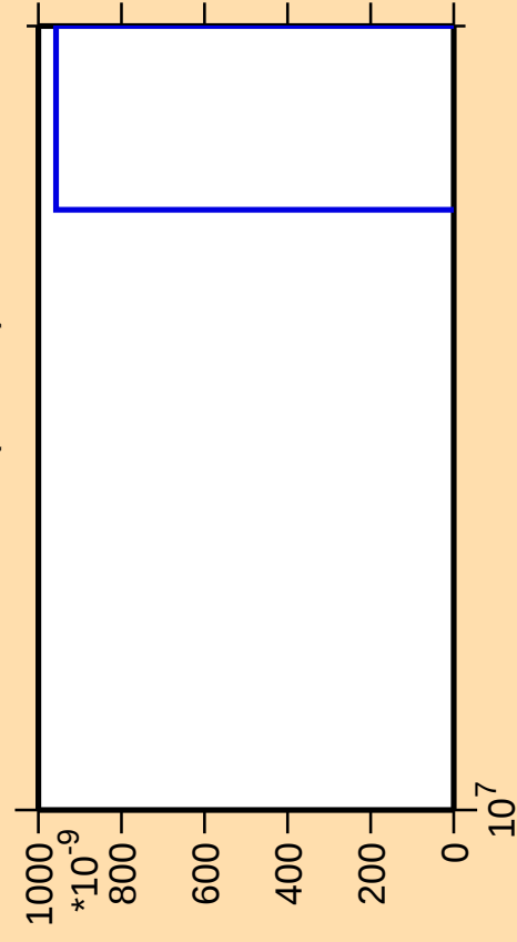
\Delta\sigma/\sigma vs. E for ^{183}\text{Pt}(\text{mt } 11)
