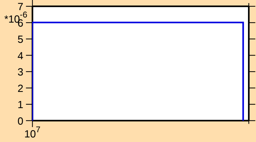
\sigma vs. E for ^{183}\text{Pt}(n,3n)
