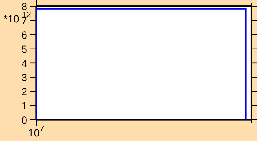
\sigma vs. E for ^{183}\text{Pt}(\text{mt117})
