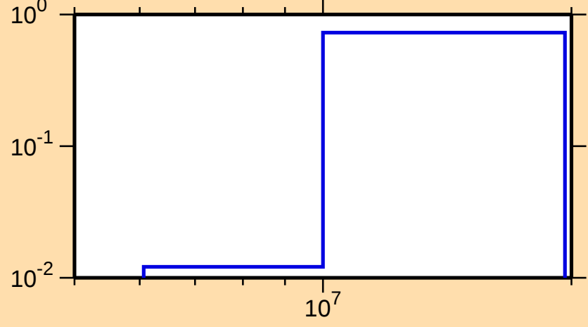
\sigma vs. E for ^{183}\text{Pt}(n,2n)
