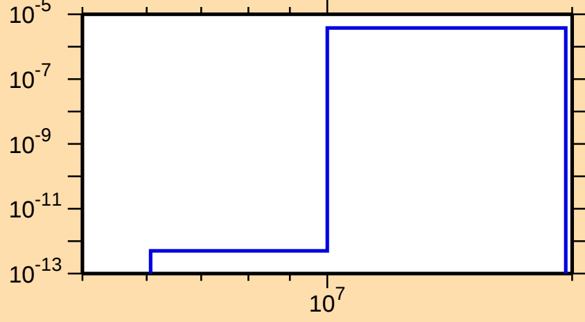
\sigma vs. E for ^{183}\text{Pt}(n,2n\alpha)
