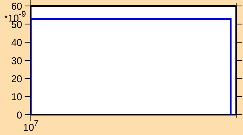
\sigma vs. E for ^{183}\text{Pt}(n,\text{nd})
