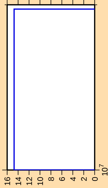
\Delta\sigma/\sigma vs. E for ^{183}\text{Pt}(n,\text{nt})
