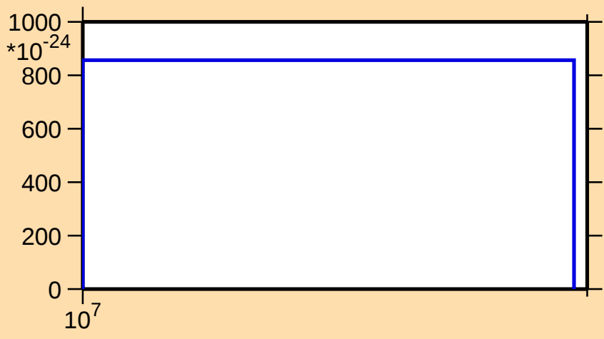
\sigma vs. E for ^{183}\text{Pt}(\text{mt } 11)
