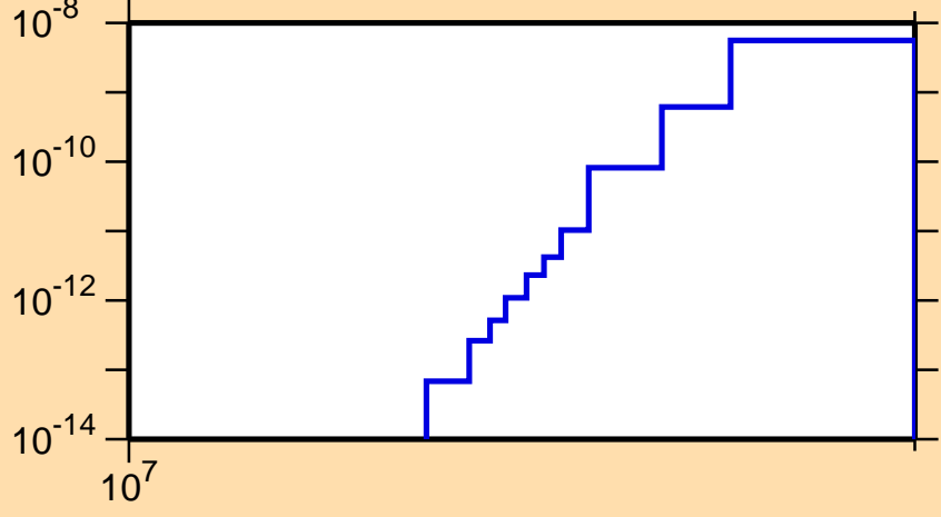
\sigma vs. E for ^{184}\text{Pt}(n,pd)
