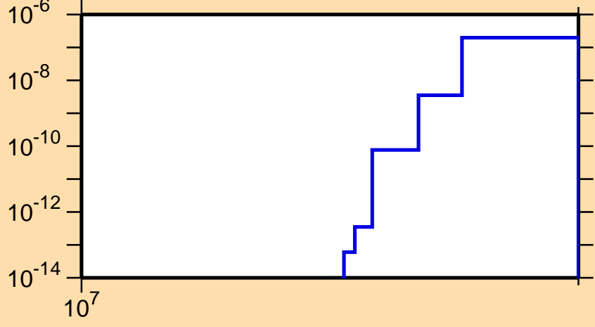
\sigma vs. E for ^{184}\text{Pt}(n,nd)
