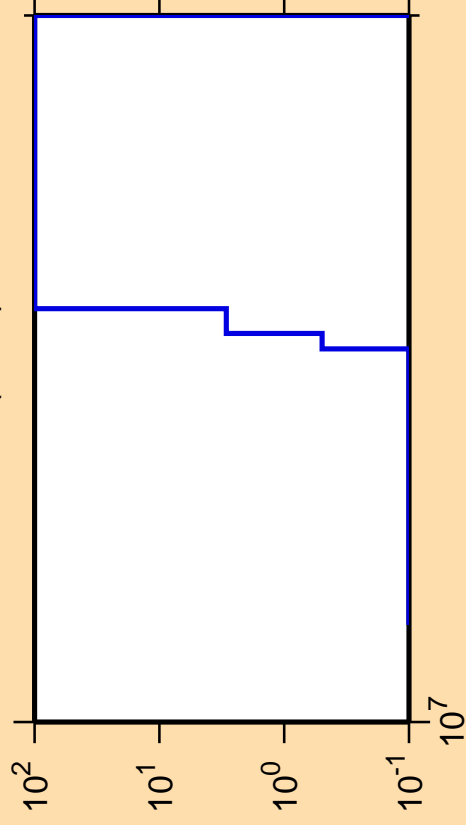
\Delta\sigma/\sigma vs. E for ^{184}\text{Pt}(n,nd)
