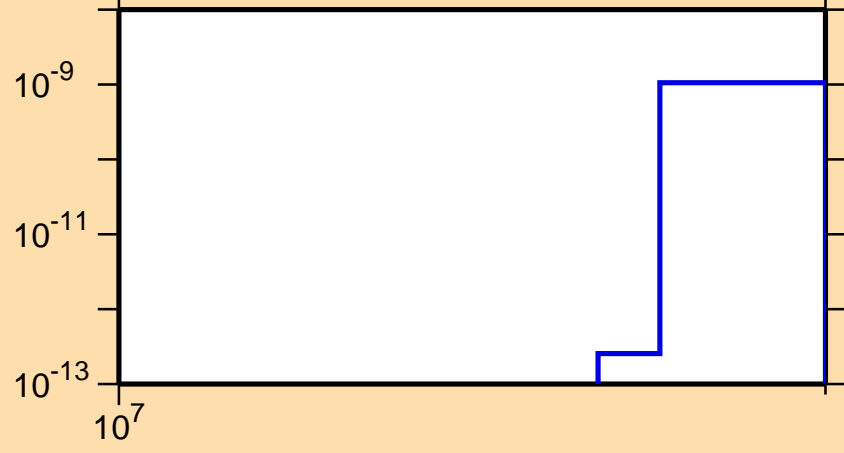
\sigma vs. E for ^{184}\text{Pt}(n,nt)
